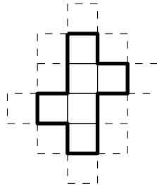
Figure 4.2: All possible adjacency empty squares on the boundary of a development of a 1 \times 1 \times 1 cube.
