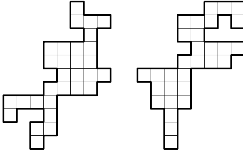
Figure 3.13: Some common developments of two boxes of size 1 \times 1 \times 7 and 1 \times 3 \times 3 .
