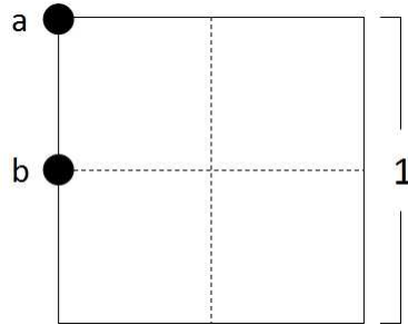
Figure 3.18: Possible locations for the center of symmetry on a unit square.
