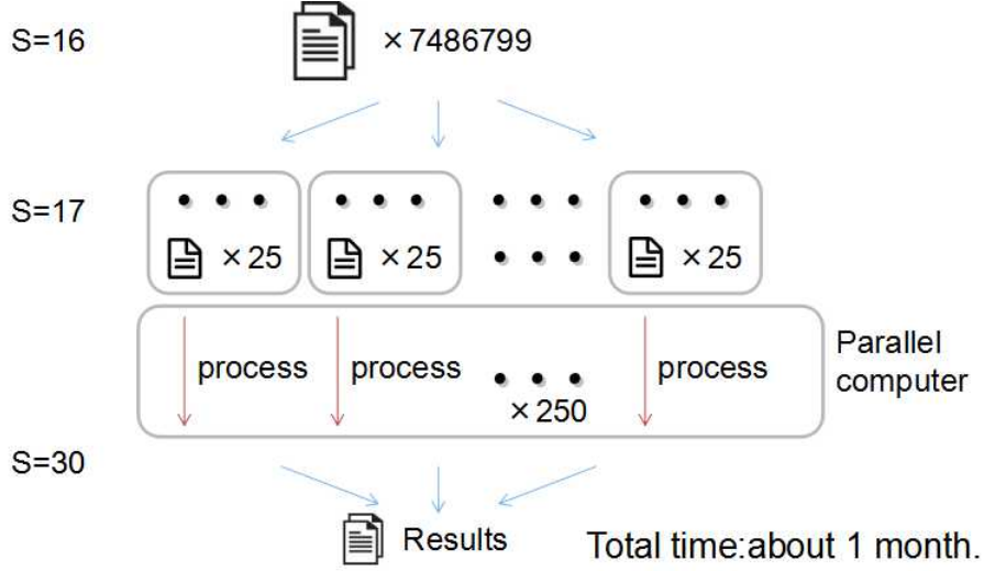
Figure 3.3: The detail of parallel computing.
