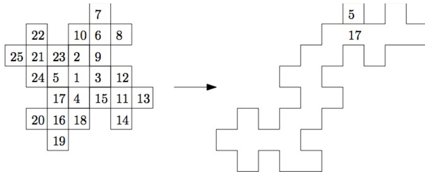
Figure 3.7: Neighbor-squares of start point marked in step 3.
