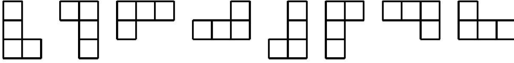
Figure 2.4: Polyominoes of the same shape.
