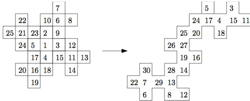
Figure 3.9: Every square is marked in step 4.
