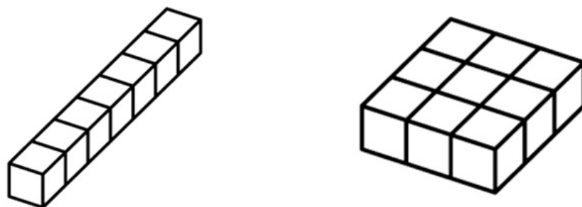
Figure 3.11: Boxes of size 1 \times 1 \times 7 and 1 \times 3 \times 3 of surface area 30.
