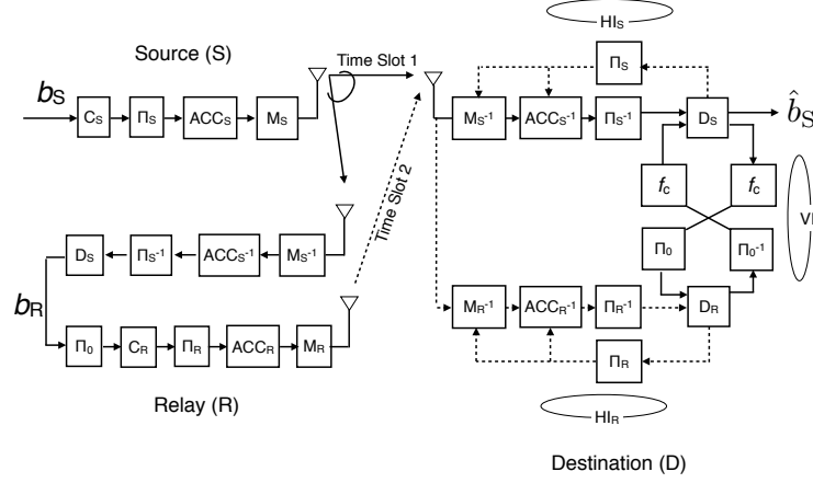
Fig. 1. Coding and decoding structure of the LF relaying system.
