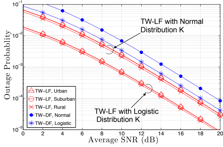
Fig. 30. Comparison of the outage probability of the two-way LF and two-way DF relaying, where R_x^c = 1 (bits/s/Hz) ( x \in (A, B) ).
