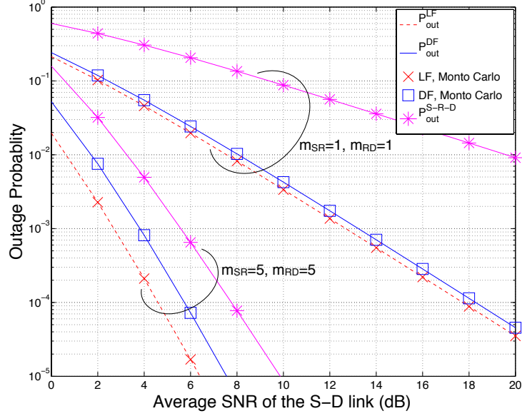
Fig. 7. Outage probability comparison among the LF, DF, and S-R-D transmission with m_{SD} = 1 .
