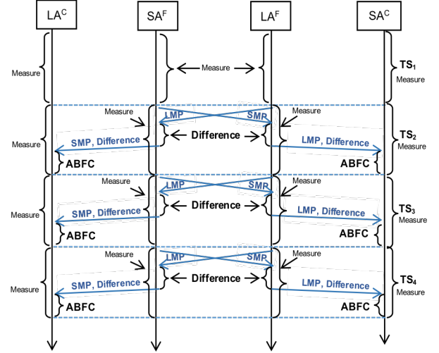
Fig. 3. Agent-Based Feedback Control Protocol.
