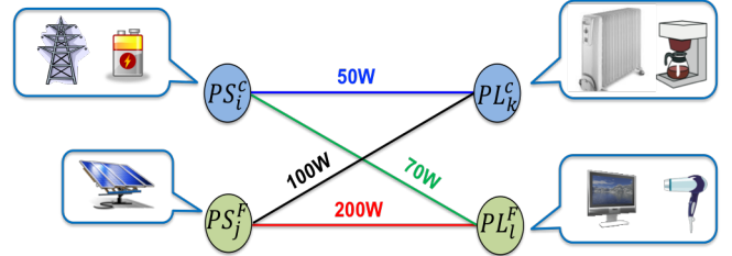
Fig. 1. Categorization of power devices: controllable and fluctuating.
