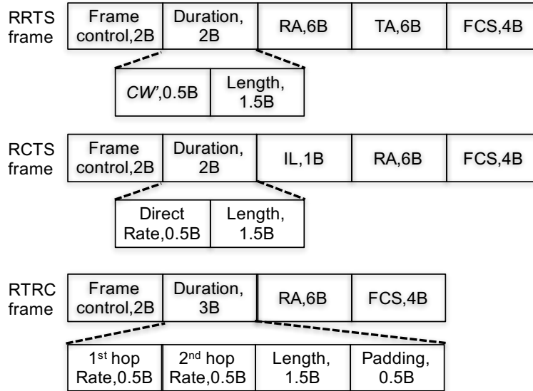
Figure 3.10: The Control Messages of NCA-2PSP Protocol
