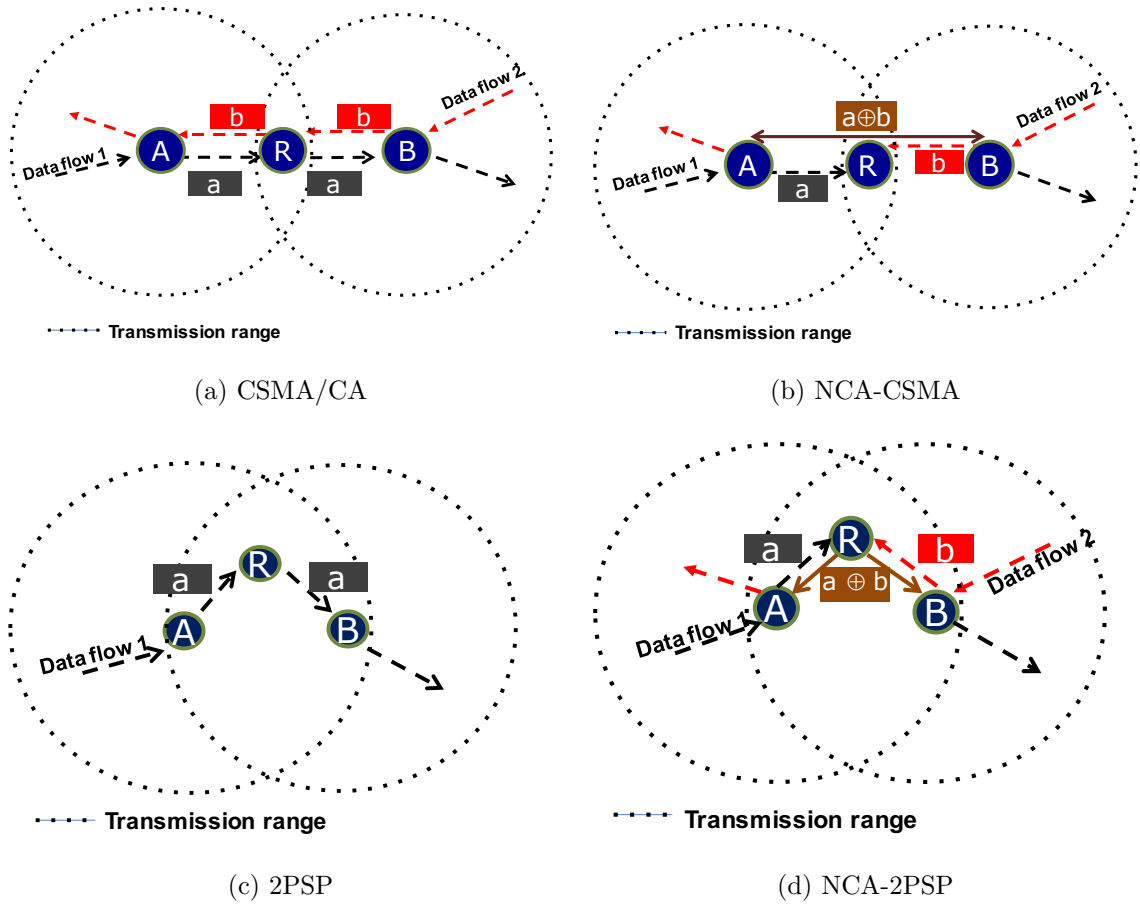
Figure 3.6: Message exchange in reference scenarios: golden chain and golden triangle topologies
