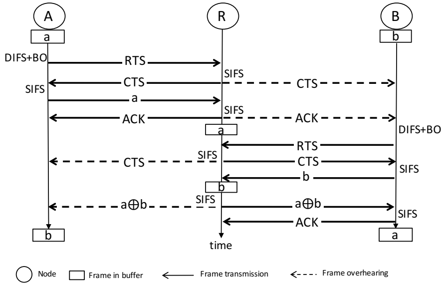
(b) Message handshaking timeline
