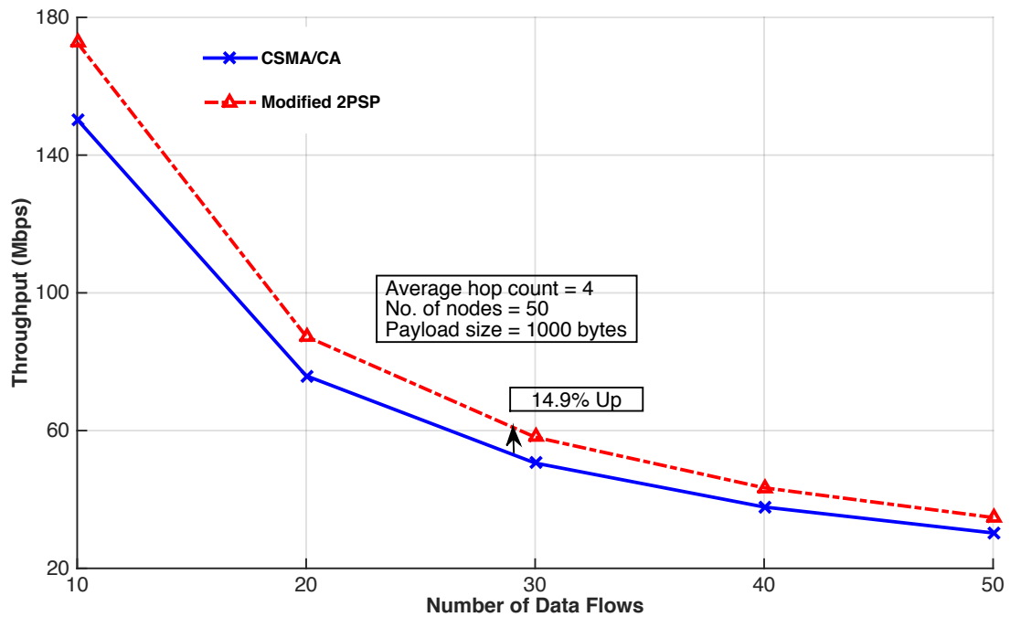
Figure 4.5: Throughput as function of flows increase
