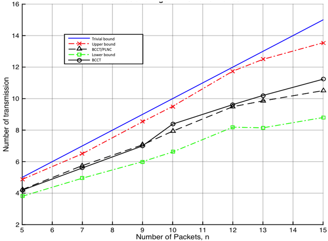
Figure 5.4: Performance of the algorithms with the increased number of messages. The client number is 5.
