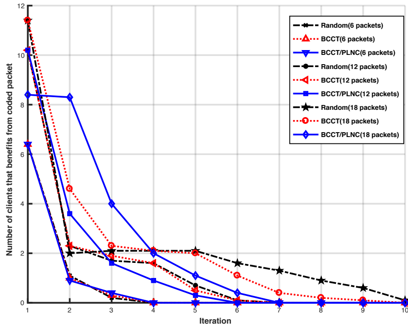
(a) Number of clients that benefits among total 14 clients for different number of messages
