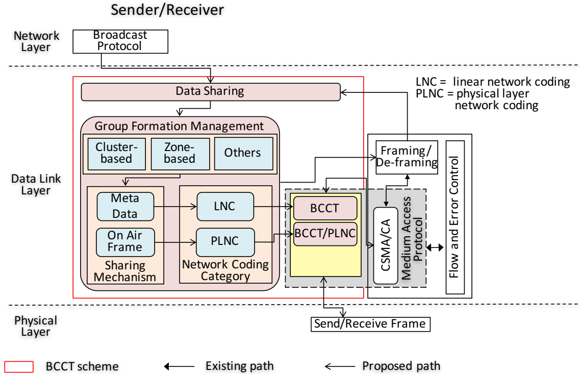
Figure 5.2: Block diagram of Balanced Cooperative Coding and Transmission (BCCT) Scheme
