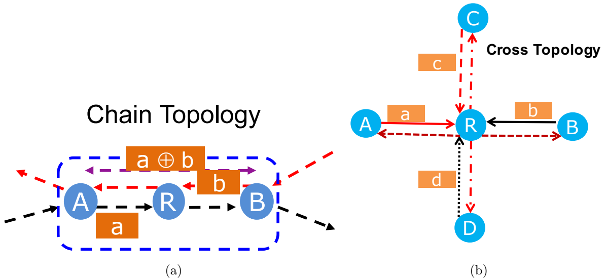
Figure 2.3: Chain topology (two-way relay channel) (b) Cross (star) topology
