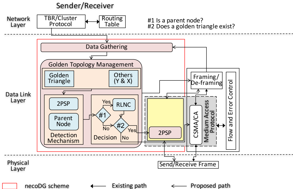
Figure 4.1: Block diagram of Network Coding-based Data Gathering (necoDG) Scheme
