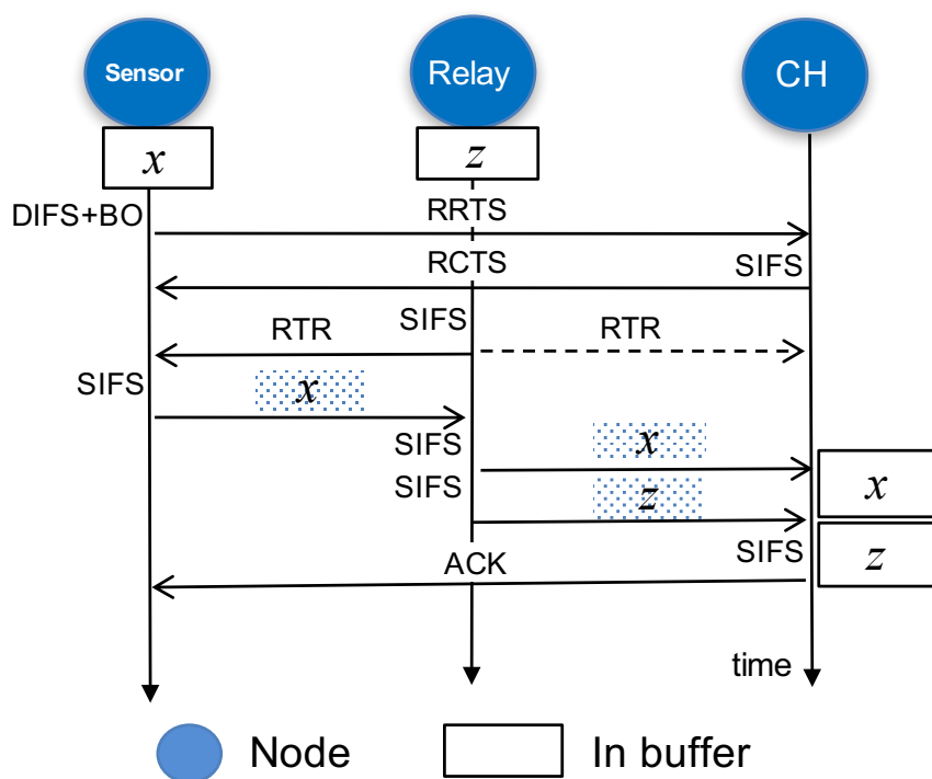
Figure 4.3: Timing operation of modified 2PSP protocol
