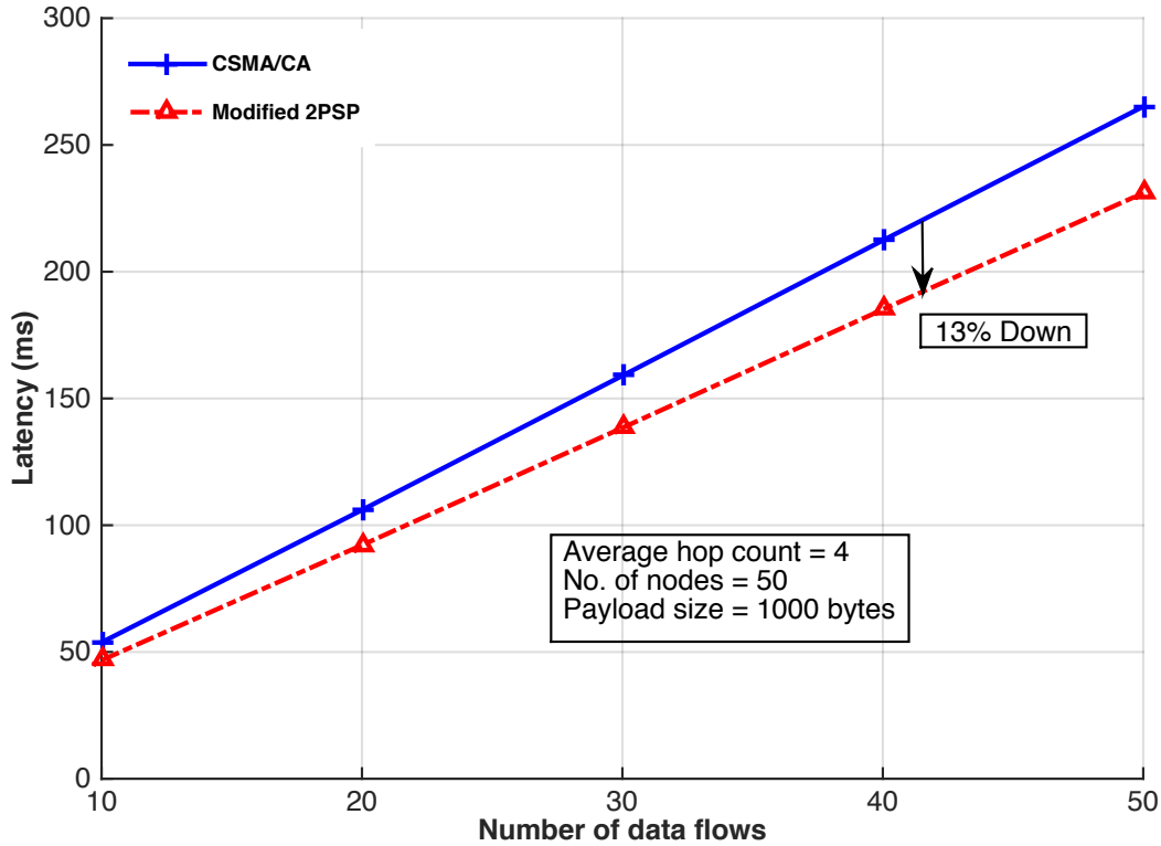
Figure 4.6: Latency as function of flows increase
