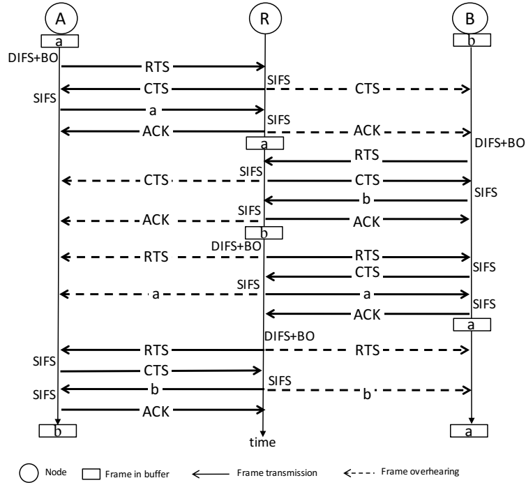
Figure 3.7: The CSMA/CA protocol message handshaking procedure for a data exchange between two nodes via a relay in a golden chain
