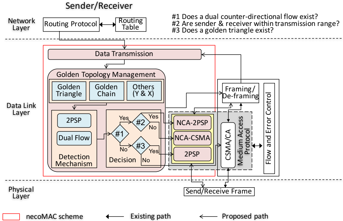
Figure 3.4: Block diagram of Network Coding-aware MAC (necoMAC) Scheme
