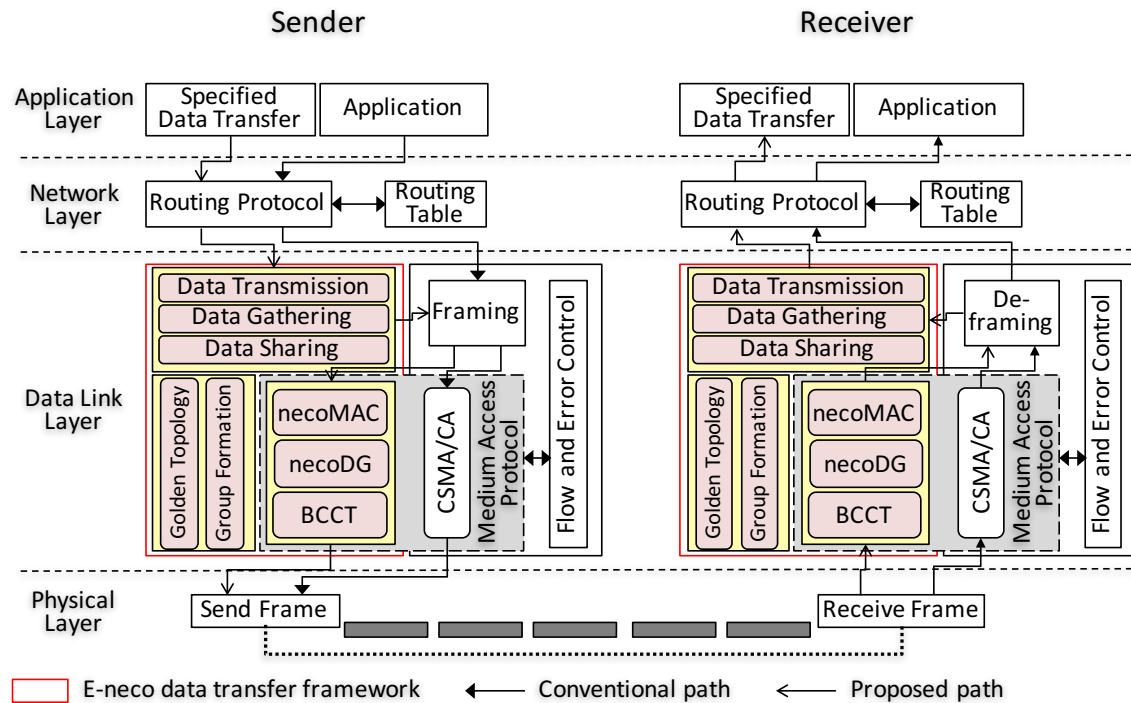
Figure 2.7: E-neco Data Transfer Framework
