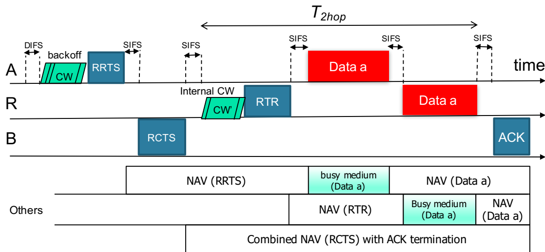
Figure 2.6: DCF message handshaking procedure of 2PSP protocol
