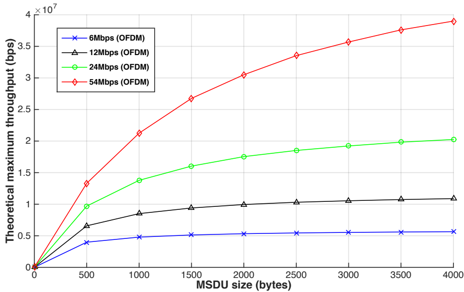
Figure 3.11: Theoretical maximum throughput curve for 802.11a OFDM RTS/CTS. The MATLAB simulator shows same performance results as in the reference.
