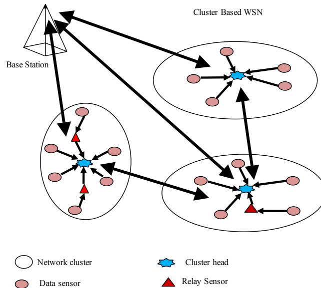
Figure 4.2: Data gathering in a cluster-based wireless sensor network (WSN)
