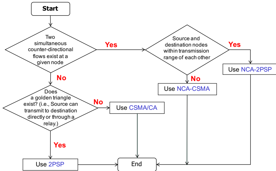
Figure 3.5: The Operation of necoMAC scheme
