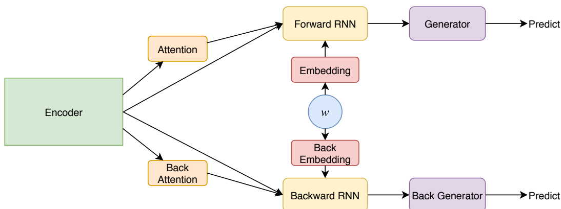
Figure 3.6: The model bidirectional decoders share no component
