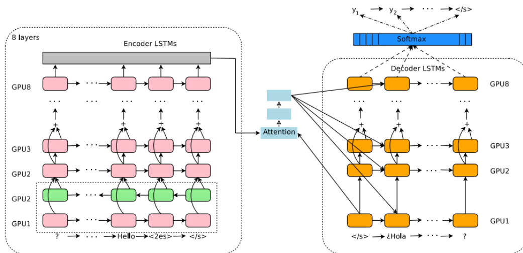
Figure 2.9: Google neural machine translation model with multi-lingual translation setting
