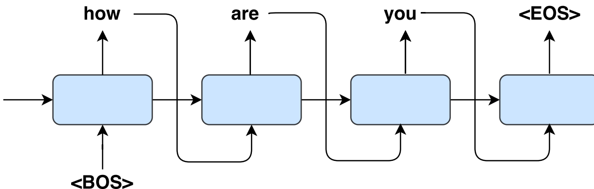
Figure 1.2: Example of unidirectional RNN decoder decoding process
