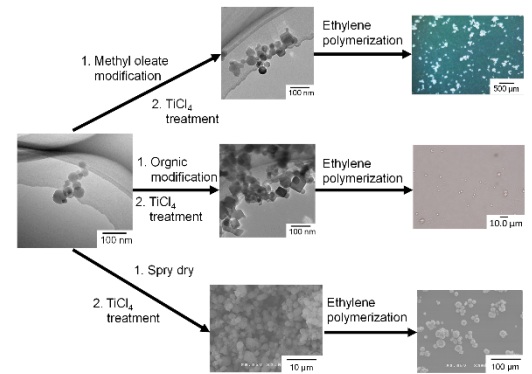
Figure 2 The synthesized UHMWPE particles.
