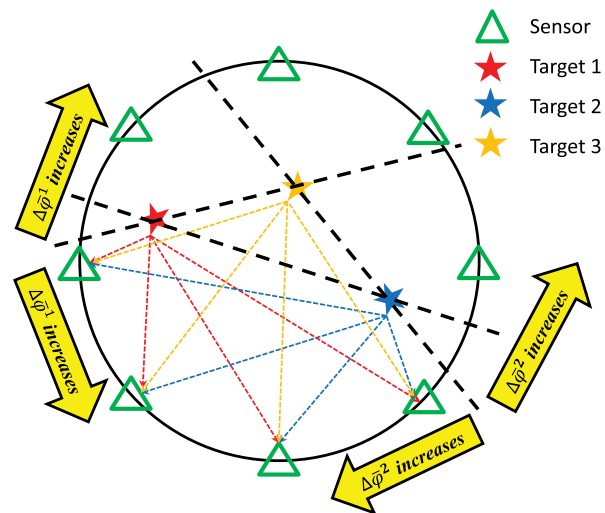
FIGURE 8. Sensor separation for 2D three-target detection.
