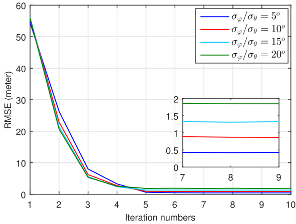
FIGURE 4. Average RMSE versus iterations for 3D single-target detection with different \sigma_\varphi/\sigma_\theta .
