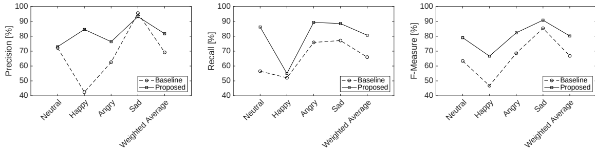
Figure 4.2: Classification results for multilingual SER obtained by different emotion theories of the baseline and proposed approaches.
