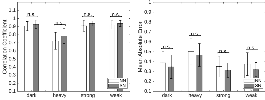
Figure 5.1: Estimation performance of semantic primitives by multilingual emotion recognition system using the proposed acoustic features with respect to SN and NN.
