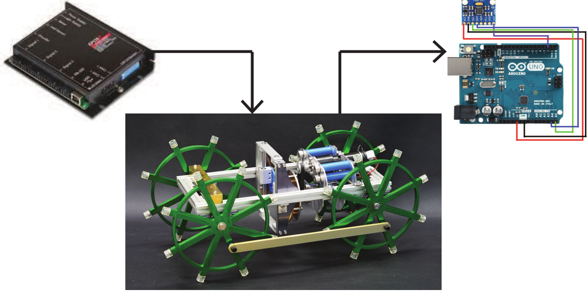
Figure 3.3: Experimental system
