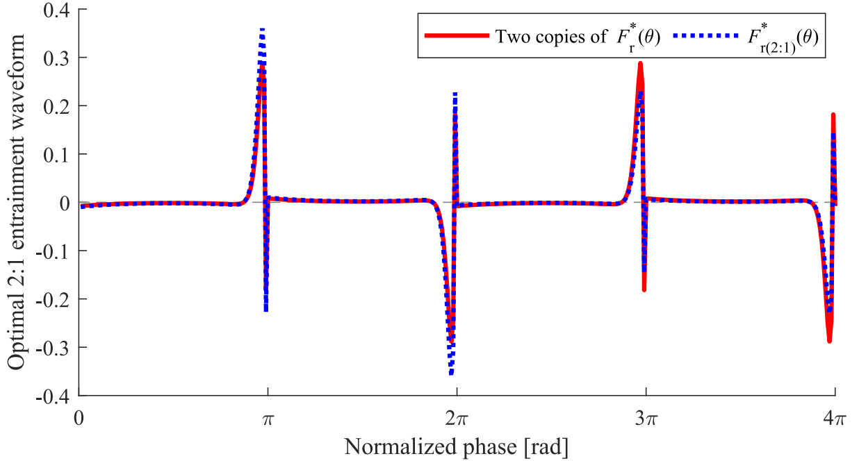
Figure 4.4: Optimal waveform for 2:1 entrainment
