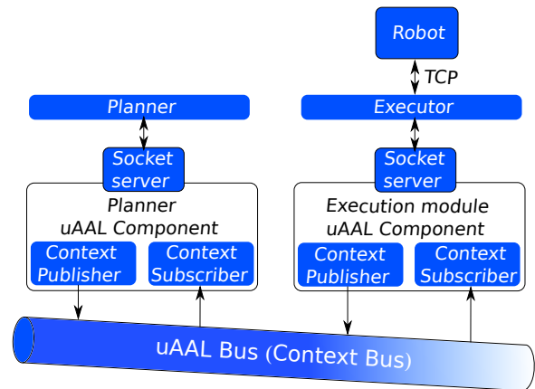
Fig. 3. Illustration of the software architecture, including the uAAL infrastructure, the planner, the executor, a robot.
