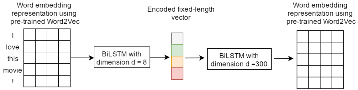
(a) BiLSTM model
