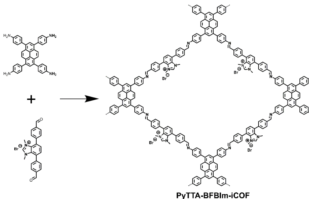
Figure 20. Imine-linked positively charged PyTTA-BFBIm-iCOF. 68
