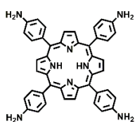
Figure 9. Typical building blocks with amino-group.
