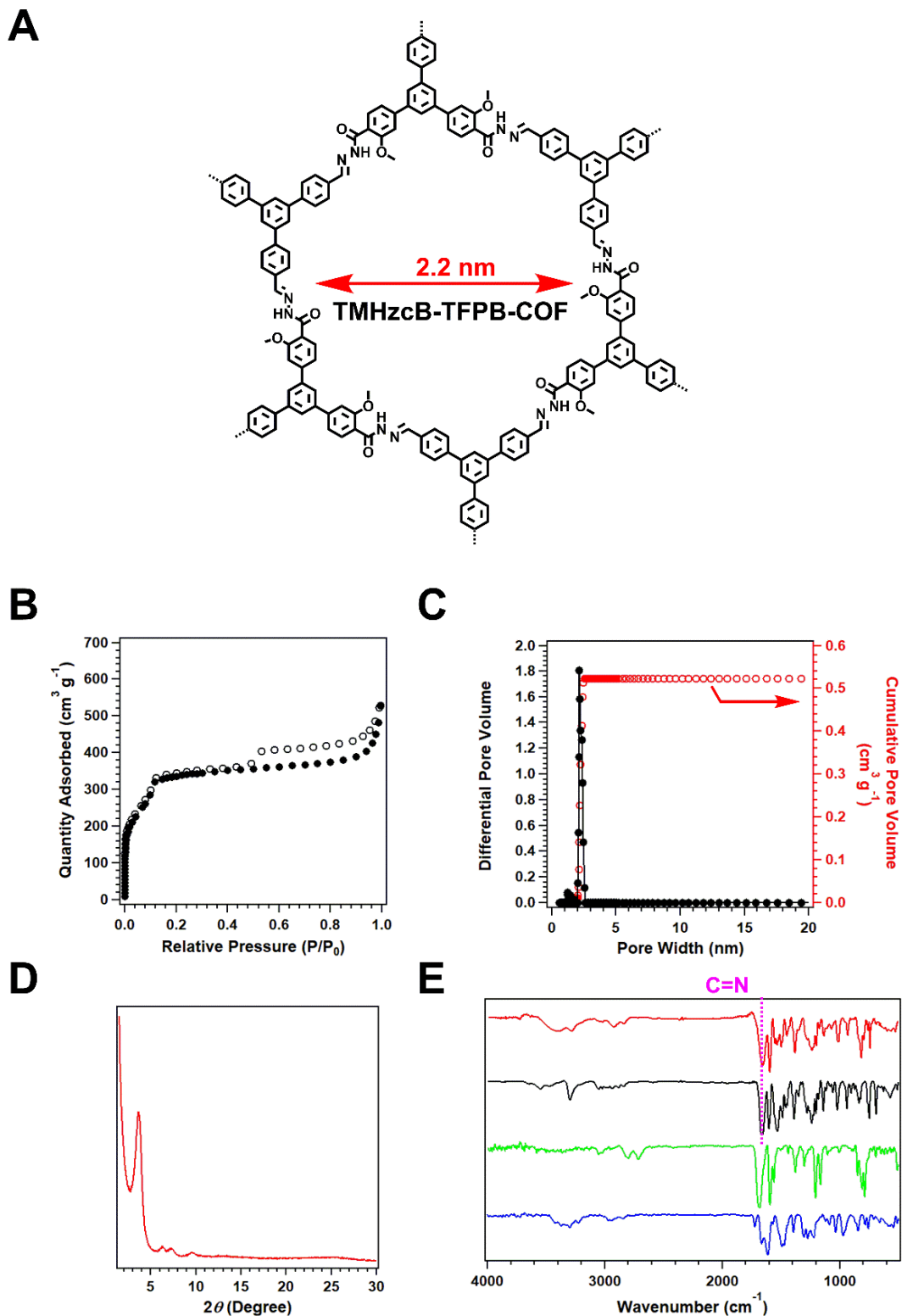
Figure 1 (A) The structure of TMHzcB-TFPB-COF. (B) Nitrogen sorption isotherm curve of TMHzcB-TFPB-COF measured at 77 K (○: desorption, ●: adsorption). (C) Pore size (black dots and curve) and pore width distribution (red dots) of TMHzcB-TFPB-COF. (D) PXRD patterns of experimentally observed. (E) FT-IR spectra of TMHzcB-TFPB-COF (red curve), Model Compound-H (black curve), TFPB (green curve), and TMHzcB (blue curve).
