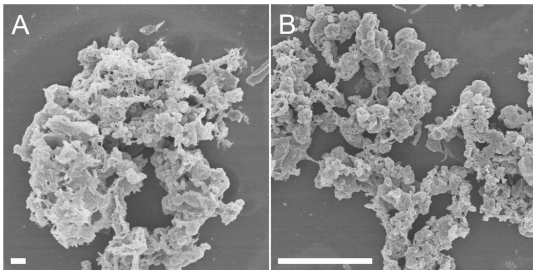
Figure 11. SEM Images of TMHzcB-2,5-DMeTA -COF (A: scale bar: 1 \mu m; B: scale bar: 10 \mu m).
