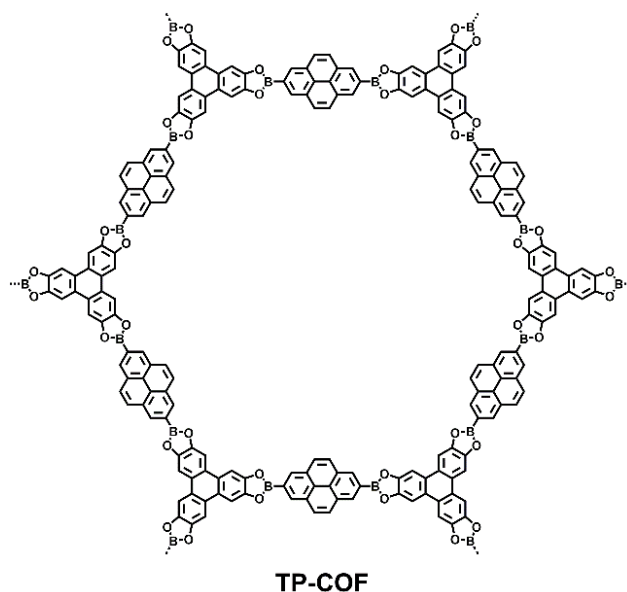
Figure 21. Structure of blue luminescence TP-COF. 70
