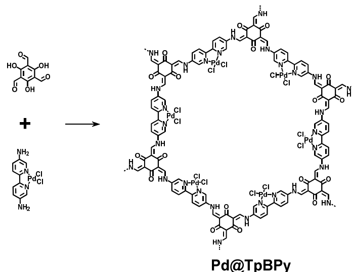
Figure 13. Synthesis and design of TpBPpy COF. 59
