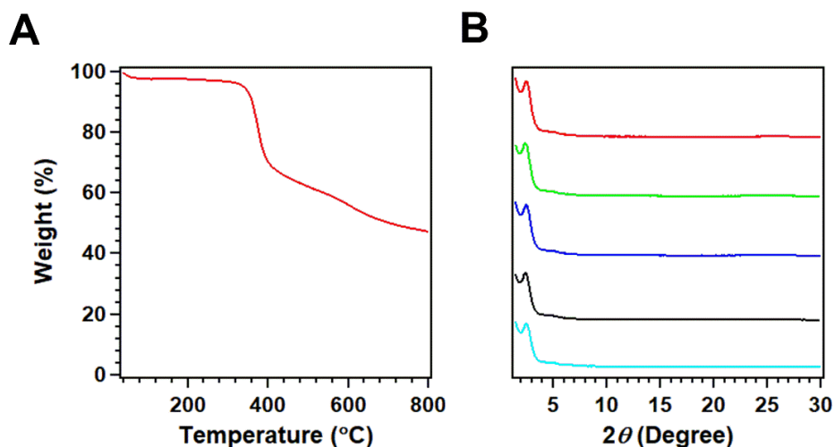
Figure 14. (A) TGA curve of TMH 2 CB-2,5-DMTA-COF under nitrogen atmosphere. (B) PXRD patterns of TMH 2 CB-2,5-DMTA-COF upon 24 h in different conditions. As-synthesized material (red line); THF (green line); water (blue line); 1M HCl (black line); 1 M NaOH (sky-blue line).
