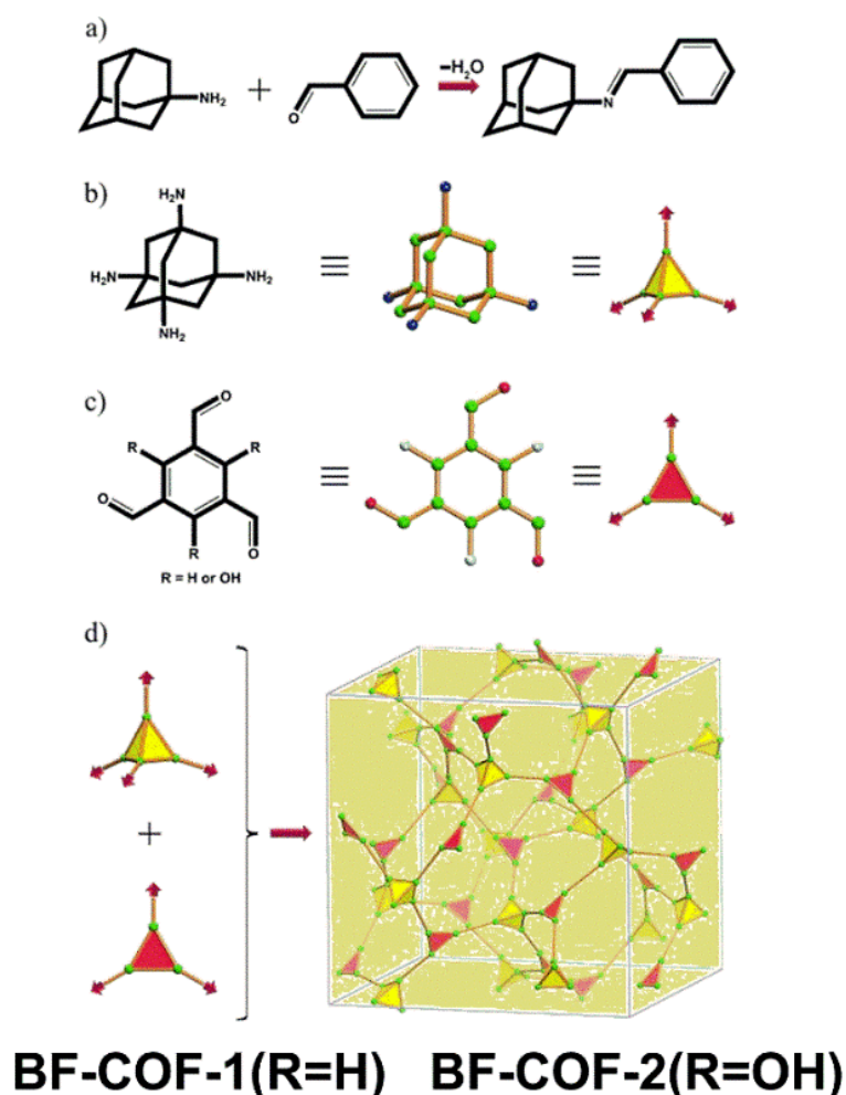
Figure 11. Design of 3D microporous COFs. (a) Model reaction of 1-adamantanamine and benzaldehyde to synthesize N-(1-adamantyl) benzaldehyde imine. (b) Structure of 1,3,5,7-tetraaminoadamantane (TAA) as a tetrahedral building unit. (c) Structure of 1,3,5-triformylbenzene (R = H, TFB) or triformylphloroglucinol (R = OH, TFP) as a triangular building unit. (d) Condensation of tetrahedral and triangular building units to give a 3D network with the symbol ctn (BF-COF-1 or BF-COF-2). 57
