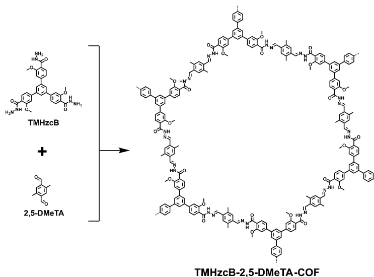
Scheme 5. Synthesis and structure of TMHzcB-2,5-DMeTA-COF.
