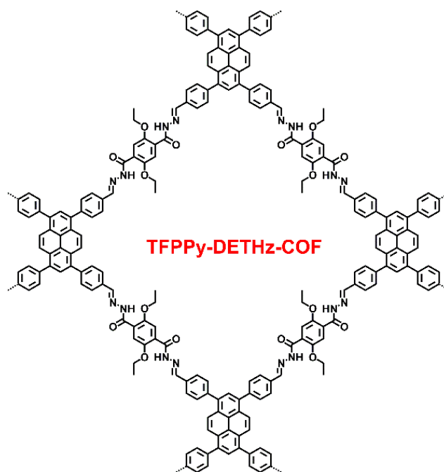
Scheme 3. Structure of TFPPy-DETHz-COF.
