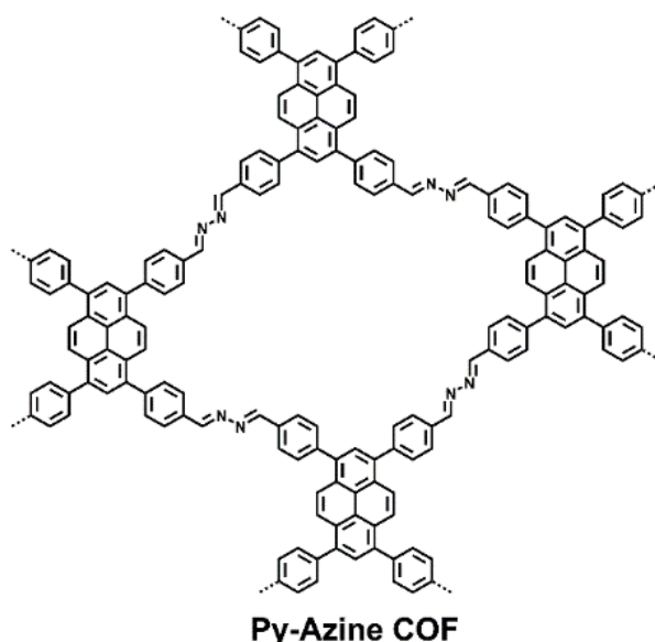
Figure 22. Structure of green fluorescence Py-Azine COF. 22
