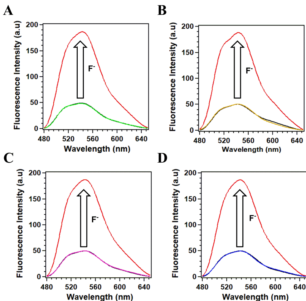
Figure 10. Fluorescence spectra of TFPPy-DETHz-COF with addition of \text{Cl}^- (A, green curve), \text{Br}^- (B, orange curve), \text{I}^- (C, purple curve), and \text{NO}_3^- (D, blue curve), followed by addition of \text{F}^- (red curves). Original COFs are black curves.
