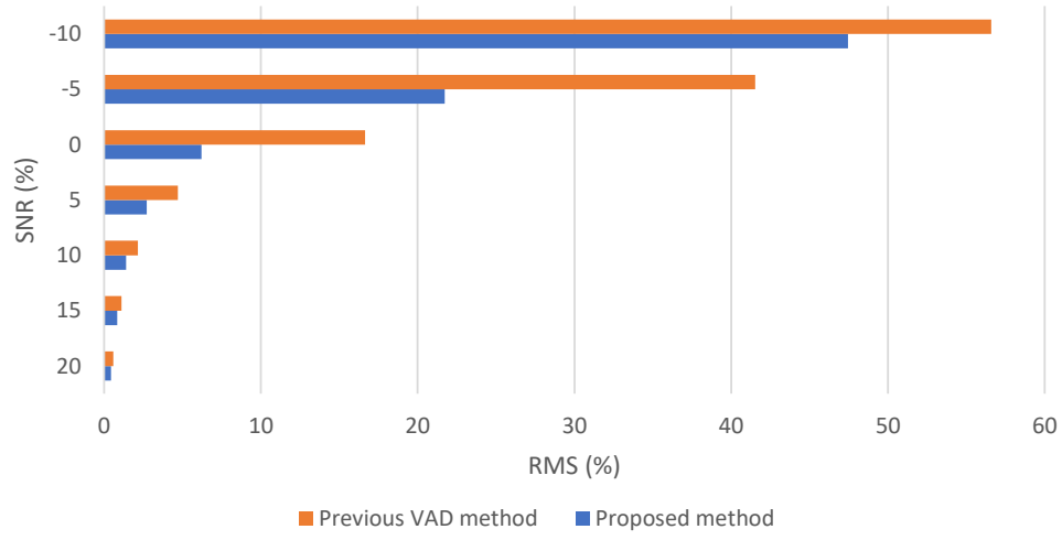
Figure 5.6: VAD Results for accuracy of RMS(%) under babble noise
