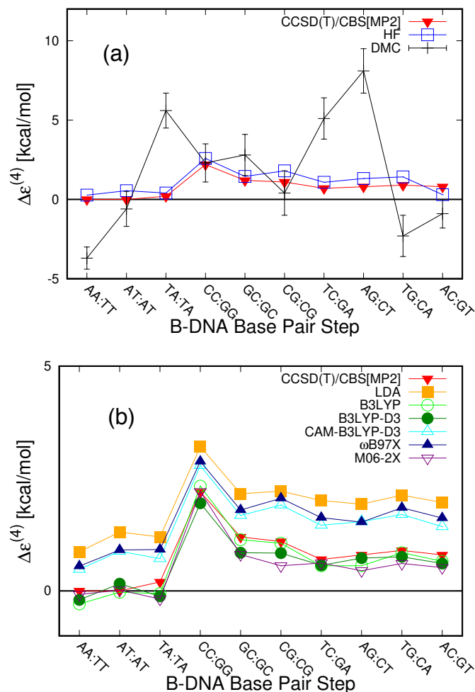
Figure 4.2: Non-additive contribution, \Delta E^{(4)} [kcal/mol], evaluated by various methods. DF-LMP2 [2] and SAPT [3] appearing in Fig. 4.1 are not shown here because their non-additive contributions are not available. For CCSD(T), the data is taken from the preceding work. [1] Unlike stacking energies (Fig. 4.1), CCSD(T) agrees with both HF and B3LYP, while it is far from FNMDC. Plausible discussions for this are given in the text.
