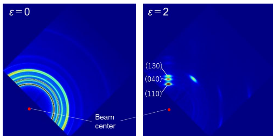
Fig. 9. WAXD patterns of PP-OTMS5 at \varepsilon = 0 and 2.
