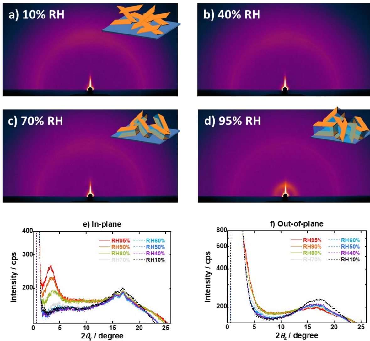
Figure 2. GISAXS results for the LM_w film. Panels a, b, c, and d respectively depict 2D GISAXS patterns at 10% RH, 40% RH, 70% RH, and 95% RH. The humidity-dependent 1D GISAXS profiles in the (e) in-plane and (f) out-of-plane directions of the Non-oriented lamellar thin film are also shown. The scattering arcs at positions of 16 and 17 deg result from diffraction of the Lumirror film used as windows for the humidity-controlled GISAXS cell.
