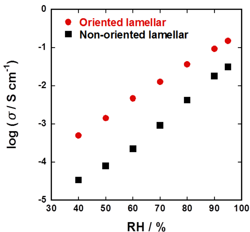
Figure 3. RH-dependent proton conductivity plots for both the Oriented lamellar and Non-oriented lamellar thin films at 298 K.
