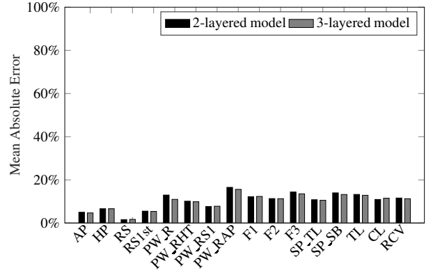
Figure 14: Mean absolute error of acoustic features from three- and two-layered model.
