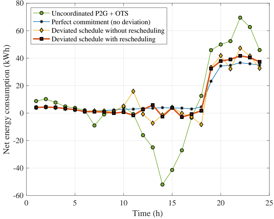
Figure 5.2: Aggregate net energy consumption profiles of 100 users in the case of uncoordinated P2G+OTS, perfect commitment, deviated schedule without and with rescheduling algorithm
