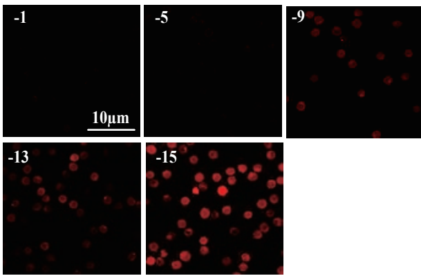
Fig. 2. CLSM images of TR-labeled lysozyme protein-loaded polyampholyte after thawing from different temperatures from -1 to -15°C, followed by ice seeding. Scale bar- 10 µm.
