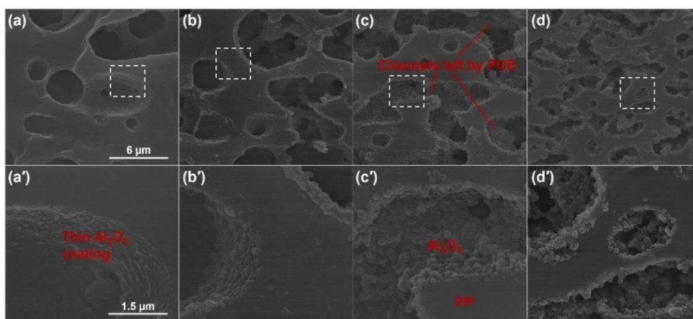
Fig. 4.4. SEM micrographs of PP/POE/Al 2 O 3 nanocomposites after the extraction of the POE phase with different Al 2 O 3 loadings: a, a') 1.2 vol%, b, b') 2.5 vol%, c, c') 5.4 vol%, and d, d') 8.9 vol%. The loading refers to the volume fraction of Al 2 O 3 nanoparticles in PP/POE/Al 2 O 3 nanocomposites before etching the POE phase. Note that the scale bar is applied to individual entire rows.
