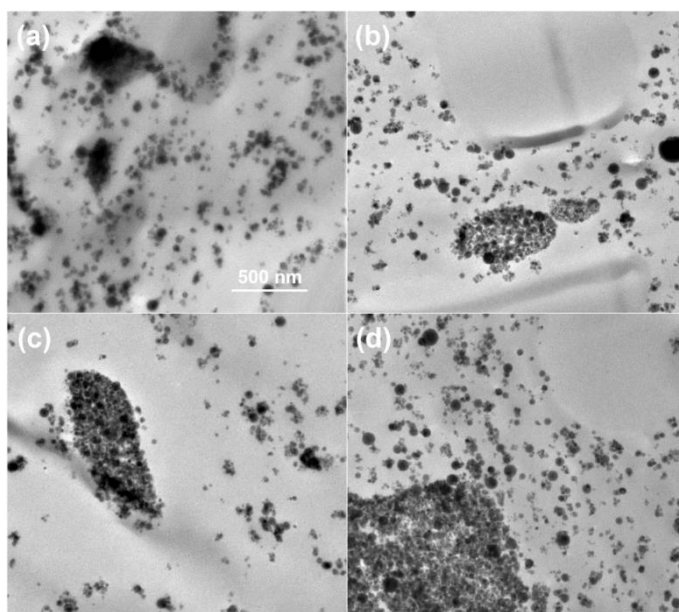
Fig. 2.13. TEM micrographs of PP/POE/ \text{Al}_2\text{O}_3 -NP nanocomposites with different kinds of POE. a) POE1, b) POE2, c) POE3, d): POE4. Note that the scale bar is applied to all the samples.
