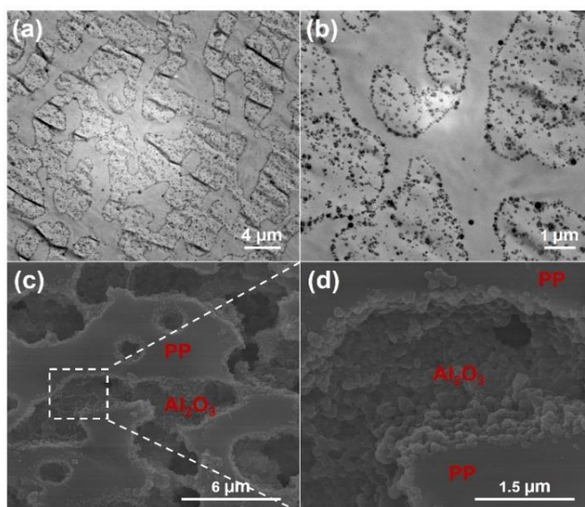
Fig. 4.2. a,b) TEM micrographs of a PP/POE/ \text{Al}_2\text{O}_3 nanocomposite with the \text{Al}_2\text{O}_3 loading of 5.4 vol% before etching. c,d) SEM micrographs of the same sample after etching the POE phase. The measurements were performed at different magnifications.
