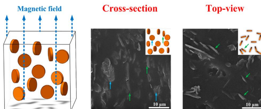
Fig. 1.7. Illustration and SEM micrographs of epoxy/hBN composites. Reproduced from Ref. [130].
