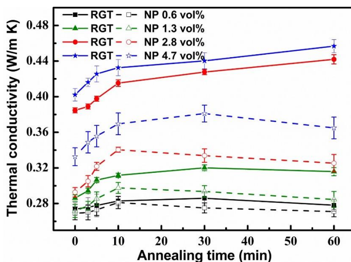
Fig. 3.9. Thermal conductivity of PP/POE/ \text{Al}_2\text{O}_3 nanocomposites annealed at 190 °C for different durations.
