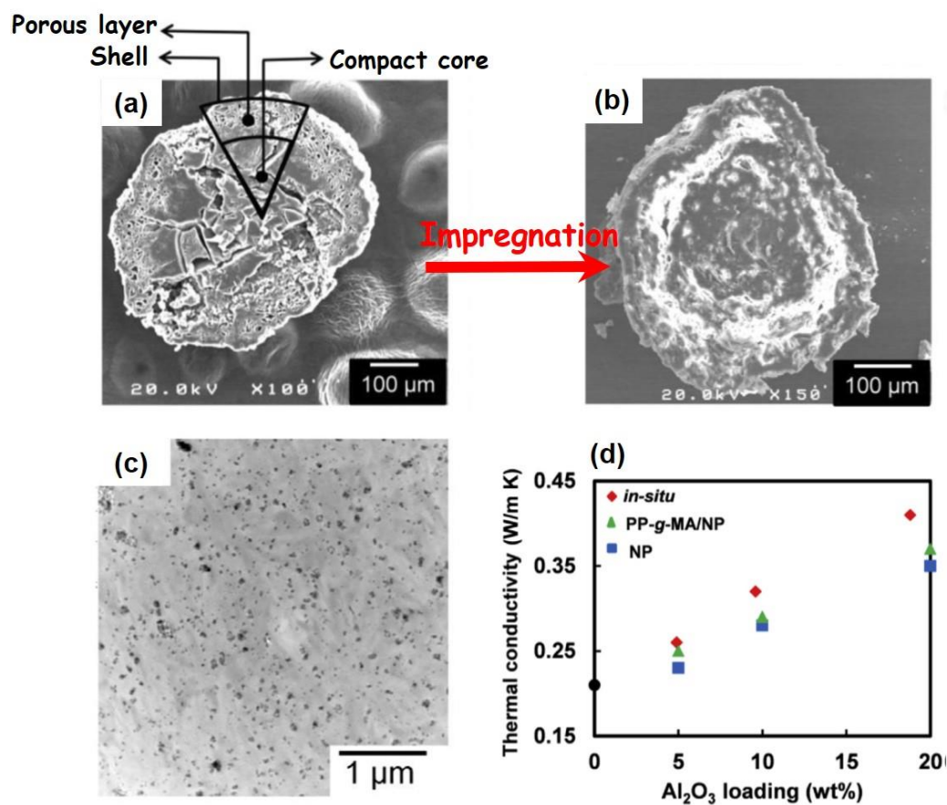
Fig. 1.18. Cross-sectional SEM micrographs of neat PP reactor granule and b) impregnated with \text{Al}(\text{O}i\text{Pr})_3 . c) TEM micrograph of the PP/ \text{Al}_2\text{O}_3 nanocomposite prepared by RGT at the \text{Al}_2\text{O}_3 loading of 20 wt%. d) Thermal conductivity of three types of PP/ \text{Al}_2\text{O}_3 nanocomposites. Reproduced from Ref. [186].
