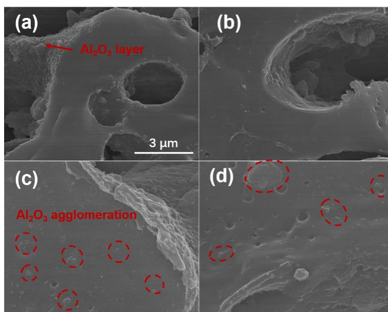
Fig. 2.8. SEM micrographs of PP/POE/ \text{Al}_2\text{O}_3 -RGT nanocomposites with different kinds of POE after selective extraction of the POE phase. a) POE1, b) POE2, c) POE3, d) POE4. Note that the scale bar is applied to all the samples.
