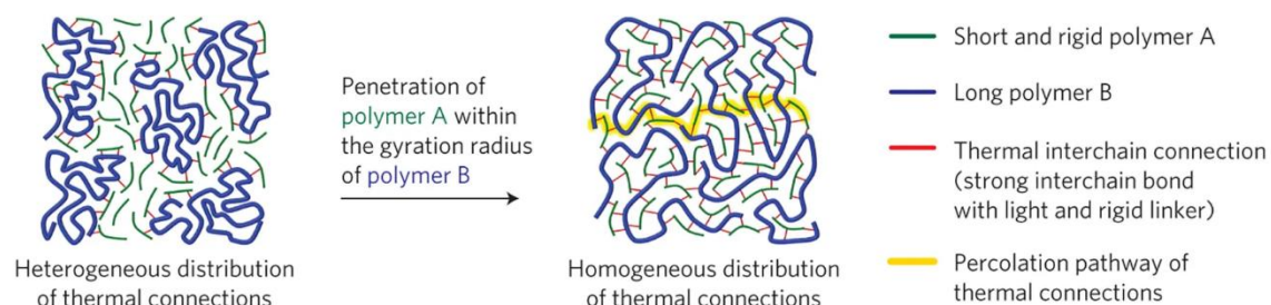
Fig. 1.2. Illustrations of heterogeneous (left) and homogeneous (right) distribution of thermal conductive interchain connections. Reproduced from Ref. [24].
