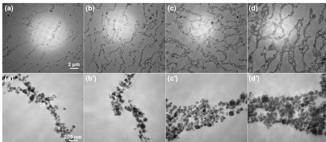
Fig. 4.9. TEM micrographs of s-PP/Al 2 O 3 nanocomposites with different loading: a) 2.2 vol%, b) 4.5 vol%, c) 9.4 vol%, and d) 14.9 vol%. a')–d') are magnified SEM micrographs. Note that the scale bar is applied to individual entire rows.
