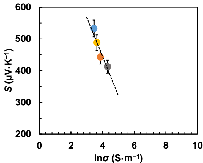
Figure 4.12. Seebeck coefficient plotted with respect to \ln(\sigma) for Pellet_1% CTS (gray circles), Pellet_3% CTS (orange circles), Pellet_5% CTS (yellow circles), and Pellet_10% CTS (sky blue circles).
