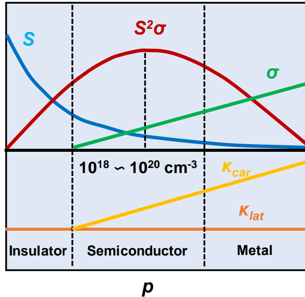
Figure 1.4. Interdependence of S , \sigma , \kappa_{\text{lat}} and \kappa_{\text{car}} on p .
