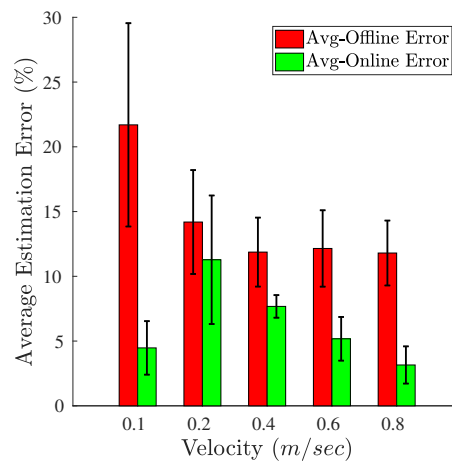
Figure 14: Range estimation error. Plot showing error in operational range calculated using the offline and online models along with corresponding standard deviation.
