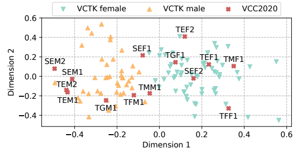
Figure 4: 2D PCA visualization of learned speaker embedding by HLE-VQVAE-3 model from VCC2020 dataset (VCC2020) and VCTK dataset (VCTK male and VCTK female). The horizontal and vertical axes are the first and second principal components, respectively.
