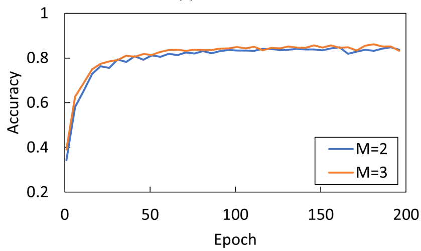
(b) CIFAR-10
