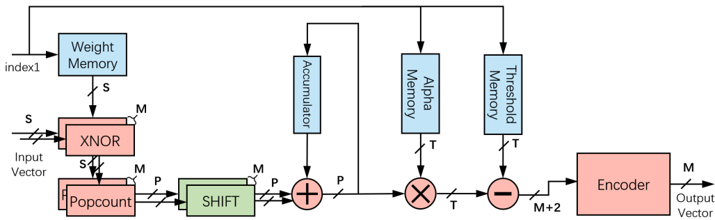
Figure 3.2: Processing Element in our design.
