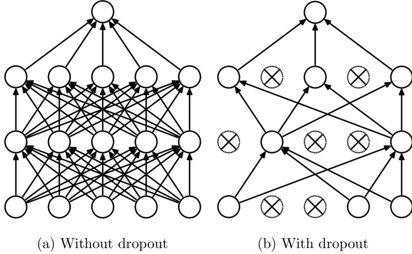
Figure 2.5: Dropout [4]
