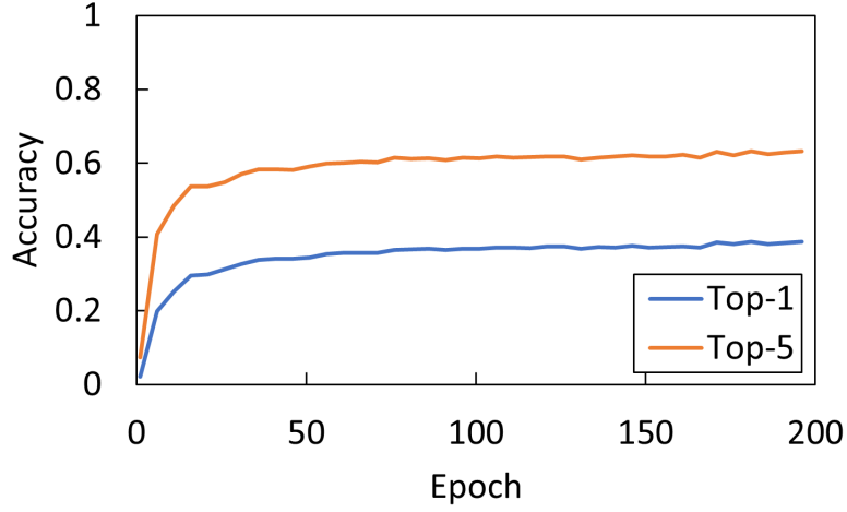
Figure 4.7: Learning Curves of ImageNet
