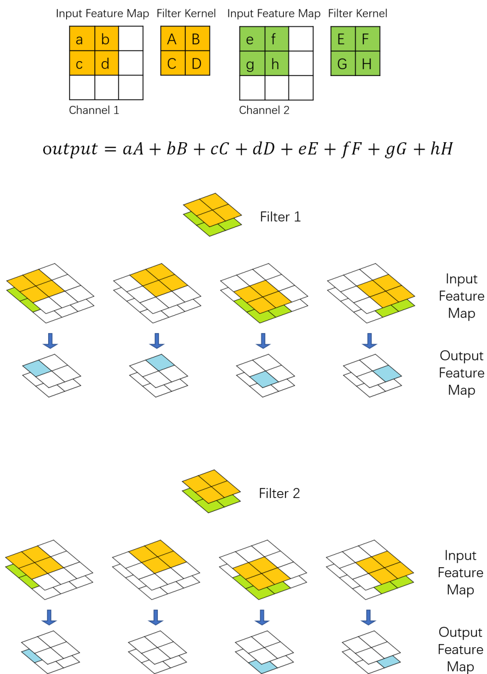
Figure 2.2: convolution operation
