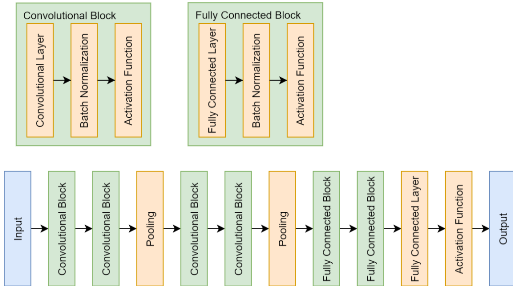
Figure 2.1: A typical CNNs model
