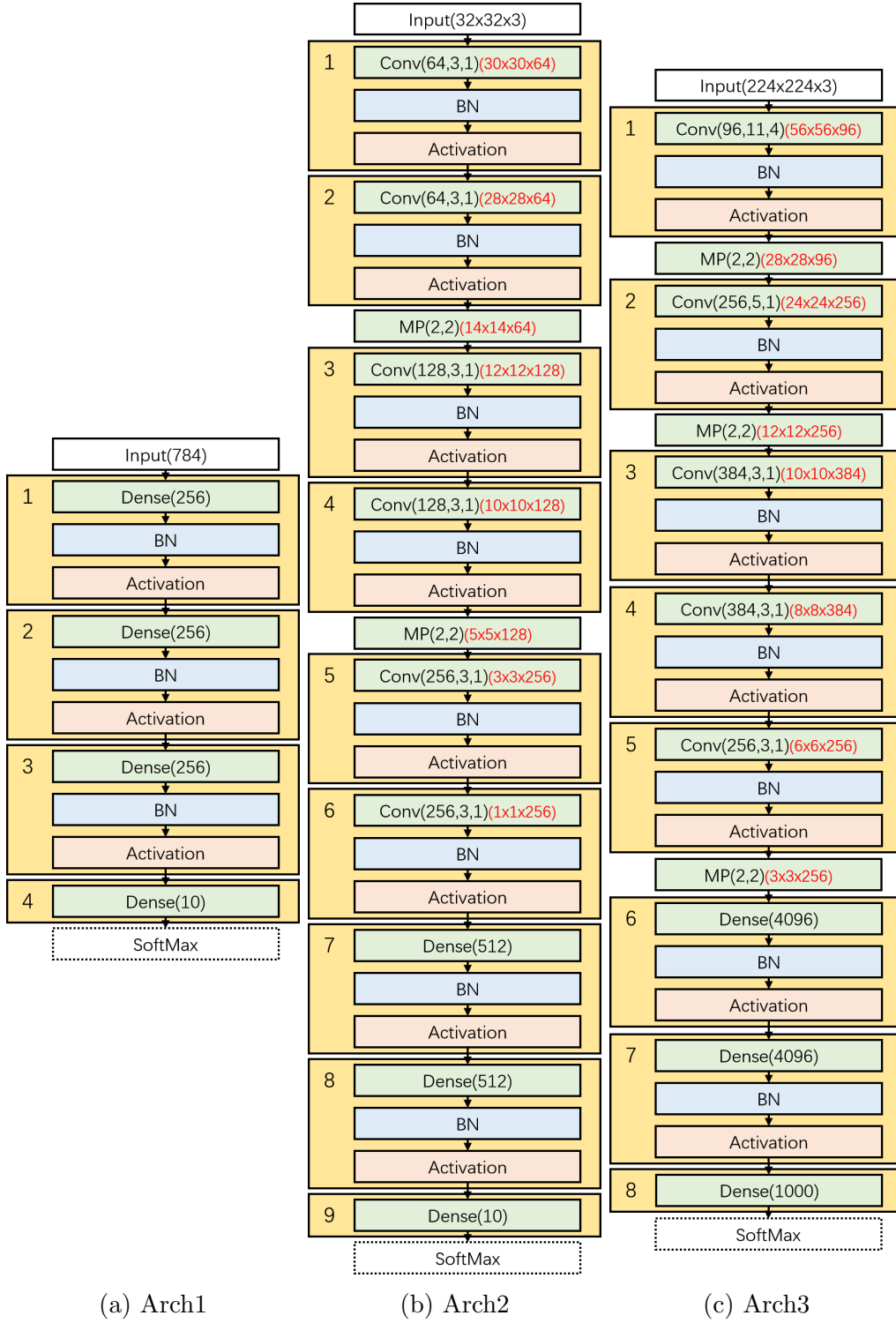
Figure 4.5: Neural Network Architectures
