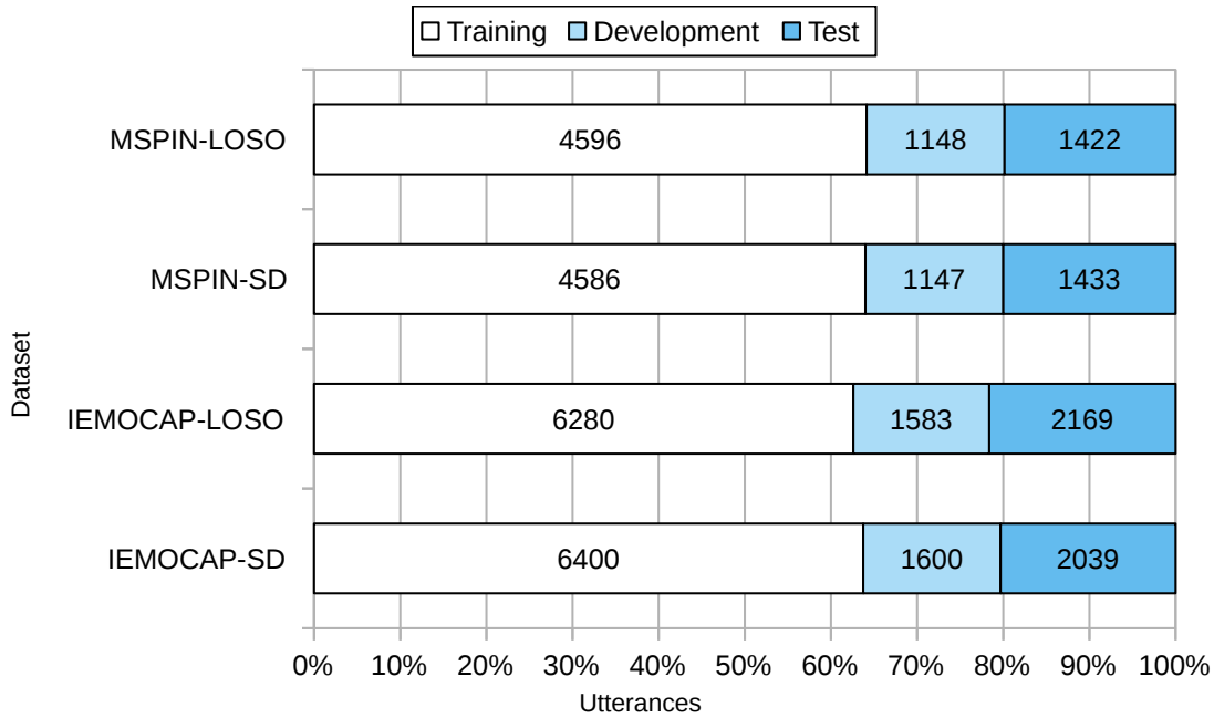
Figure 6.1: Proportion of data splitting for each partition of each dataset. In one-stage LSTM processing, the outputs of the model are both development and test data. In the second stage, i.e., the SVM processing, the input data is the prediction from the development set of the previous stage, and the output is the prediction of test data.
