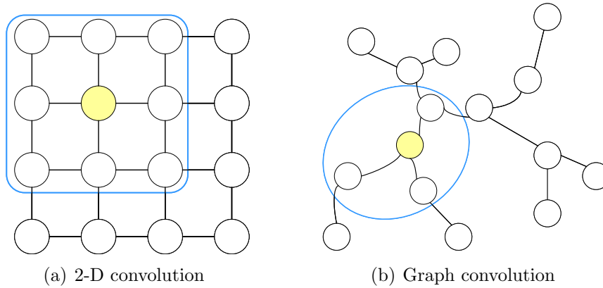
Figure 2.5: Euclidean Structure versus Non-Euclidean Structure.
