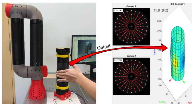
Fig. 1. The proposed TacLINK with tactile force sensing for robot links.
