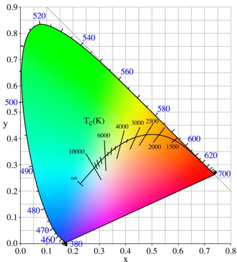
Figure 3-9. CIE chromaticity diagram with black-body curve.
