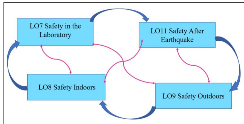
Figure 27: Interrelated LOs
