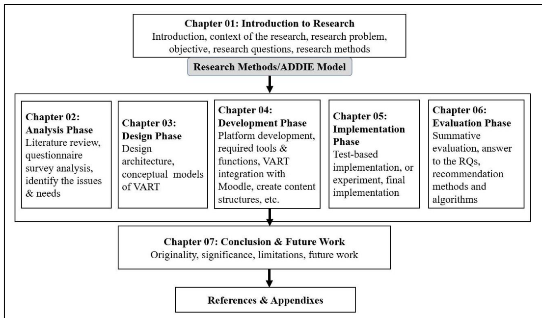
Figure 2: Dissertation structure
