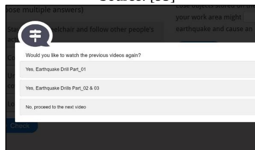
Figure 33: Decision-based path
