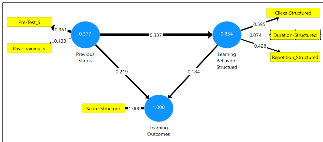
Figure 43: SEM-Structured video
