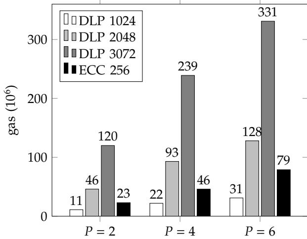
Fig. 3: Gas usages of 1024-, 2048-, 3072-bit DLP and 256-bit ECC
