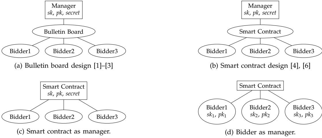
Fig. 1: (a) and (b): Traditional design. (d): our proposal. Note that (c) doesn't work since smart contract does not have secret storage.
