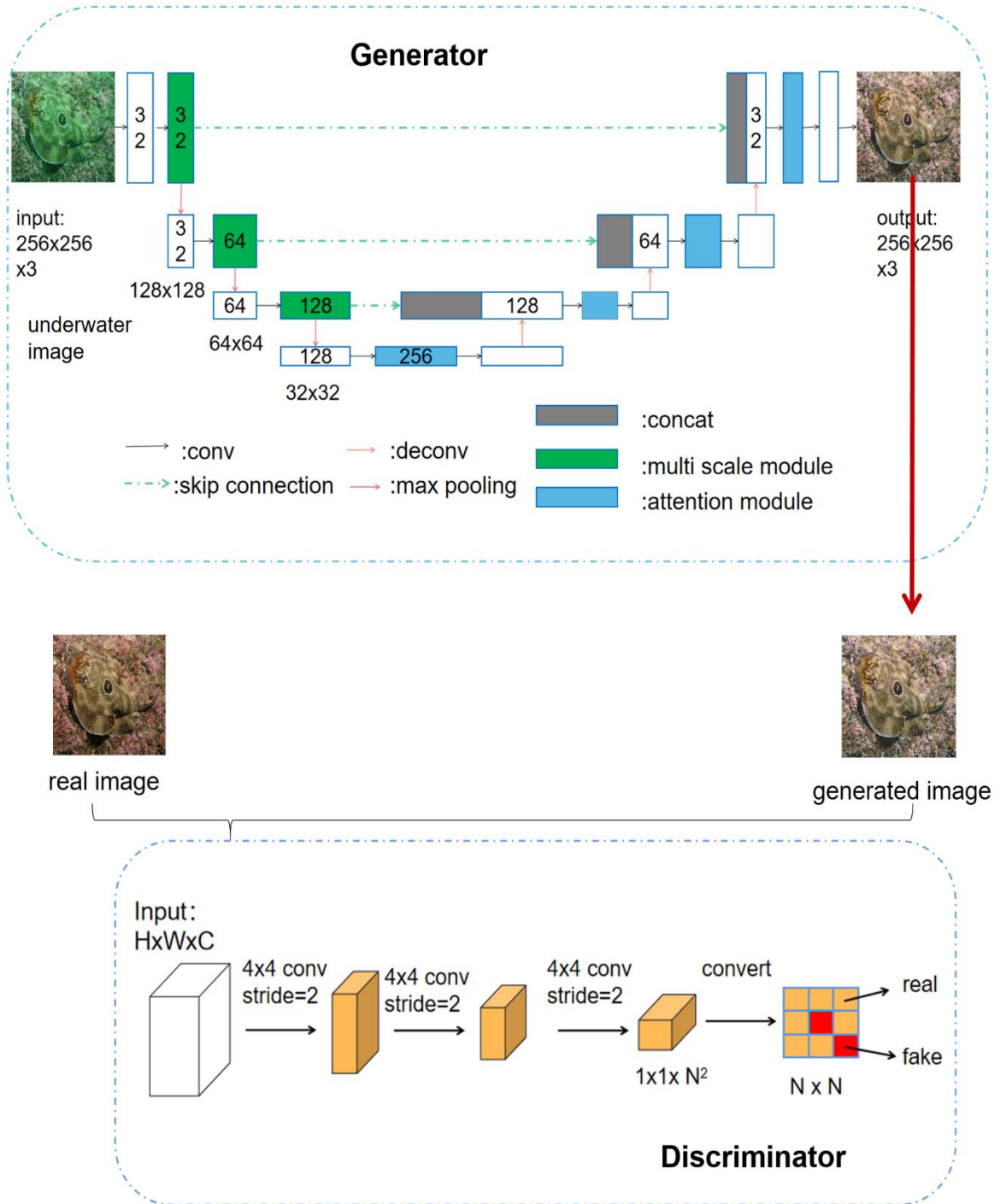
Figure 3.25: The network structure of our GAN
