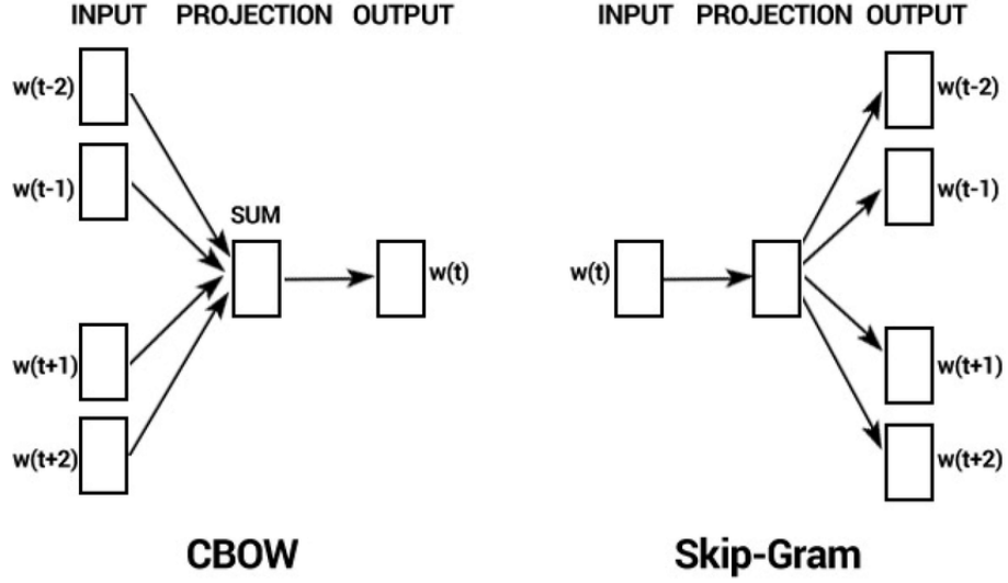
Figure 2.3: CBOW model and Skip-gram model [3]
