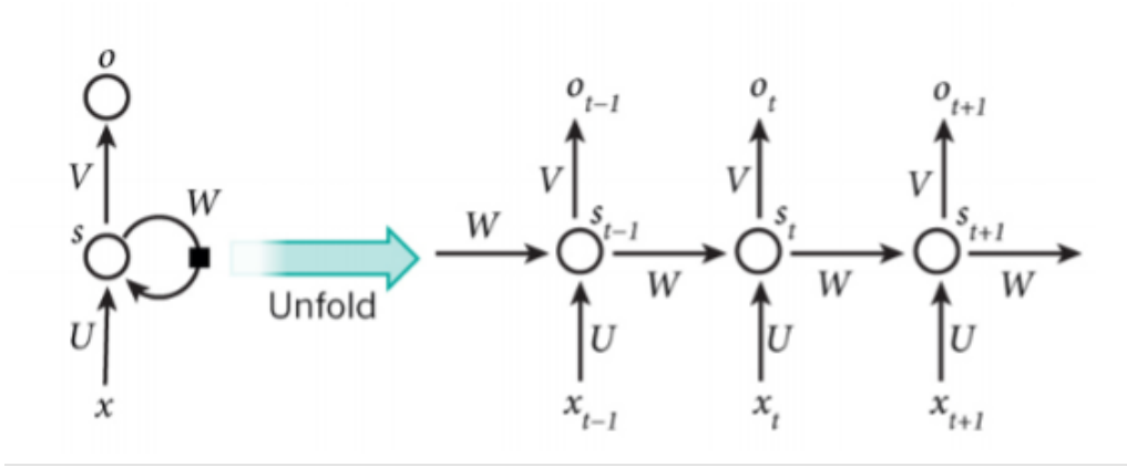
Figure 2.1: RNN structure [1]
