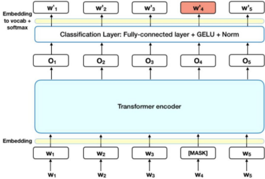
Figure 3.2: MLM model. [9]
