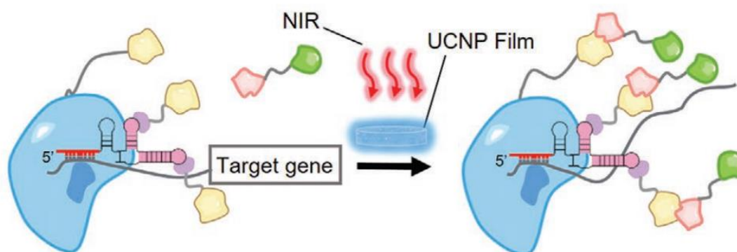
Figure 1.17 Spatiotemporal regulation of CRISPR-Cas13 by blue light irradiation
