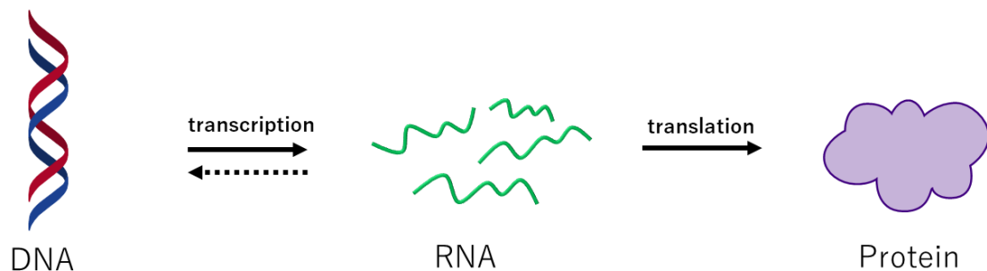
Figure 1.4. Centraldogma
