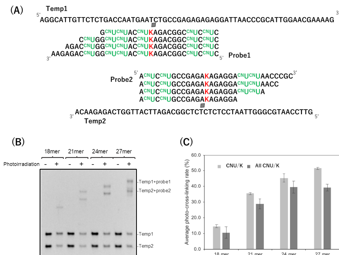
Figure 3.9. (A) DDI probe with all thymine replaced with C NU (18 mer, 21 mer, 24 mer, 27 mer). (B) Each 100 nM template strand in 10 mM Tris HCl buffer (pH 7.4) were incubated at 37 °C for 10 min followed by addition of 10 μM each probes solution incubated at 37 °C in
