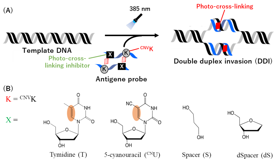
Figure 3.3. (A) DDI scheme using \text{CNV}K and self-photo-cross-linking inhibitor. (B) Self-crosslinking Inhibitor (T, \text{CNV} , dSpacer, Spacer) examined in this study.
