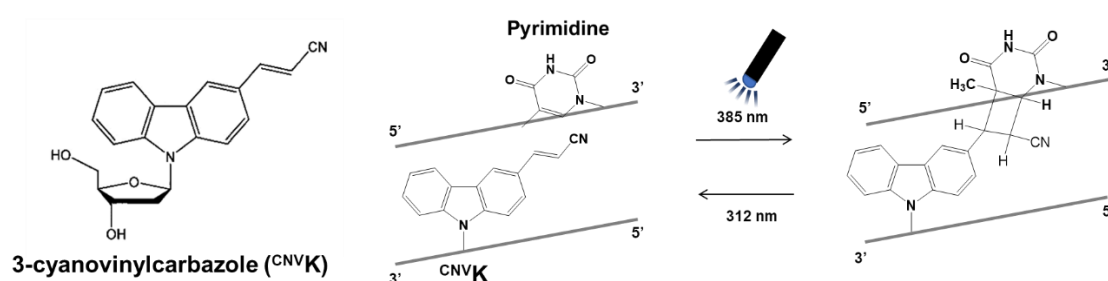
Figure 1.22 Chemical structure of CNV K and photo reversible reaction of CNV K
