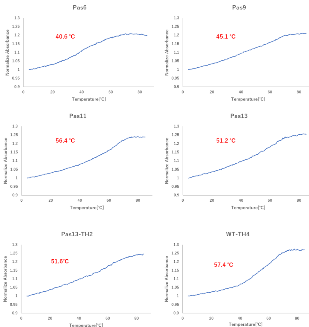
Figure 2.15. Melting curve of each DNzyme. Sample solutions were prepared by mixing 10 \mu M DNzyme and buffer (50 mM Tris-HCl (pH = 7.5) containing 200 mM KCl and 100 \mu M \text{ZnCl}_2 ). The Melting curve was analyzed at 260 nm, 85 ^{\circ}\text{C} to 4 ^{\circ}\text{C} using uv-vis spectrophotometer.
