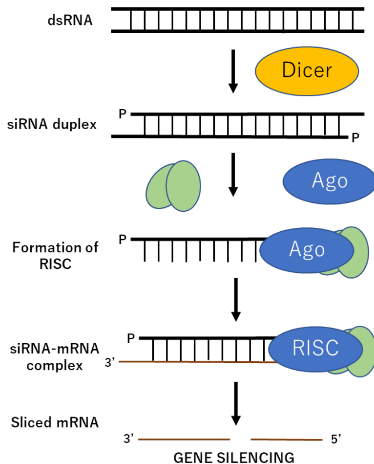
Figure 1.11 siRNA method
