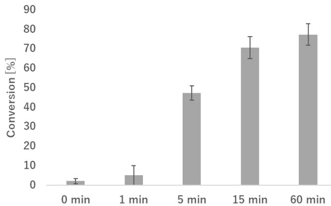
Figure 4.5. (A) Time course of incubation time using 11bp-5nt and target DNA. (0 to 60 min). (B) DDI efficiency was calculated by the template band and remaining template band.
