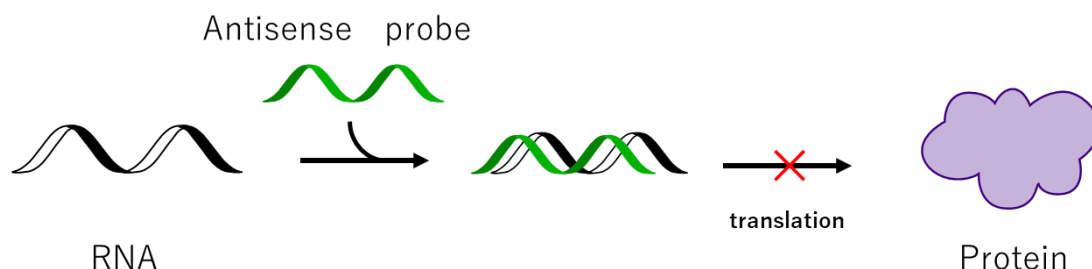
Figure 1.10. Antisense method
