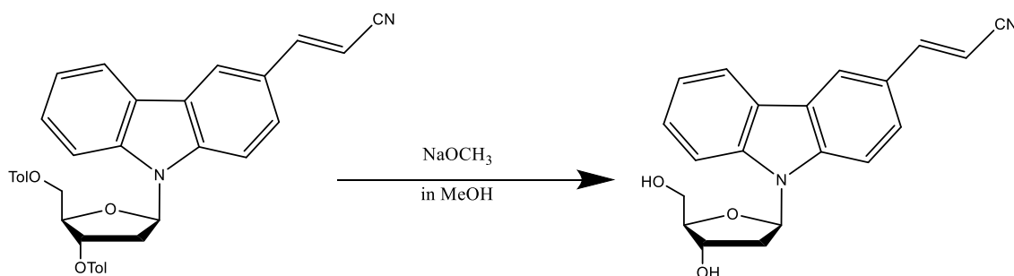
Figure 2.7. Synthesis scheme of 3-cyanovinylcarbazole-1'- \beta -deoxyribose
