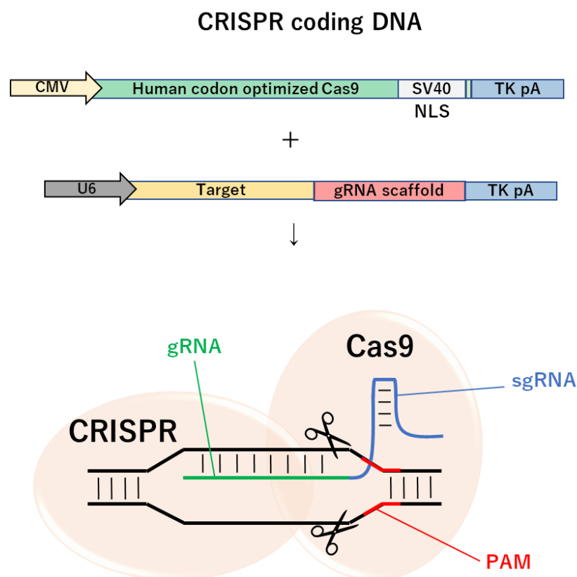
Figure 1.16 DNA cleavage scheme by CRISPR-Cas9
