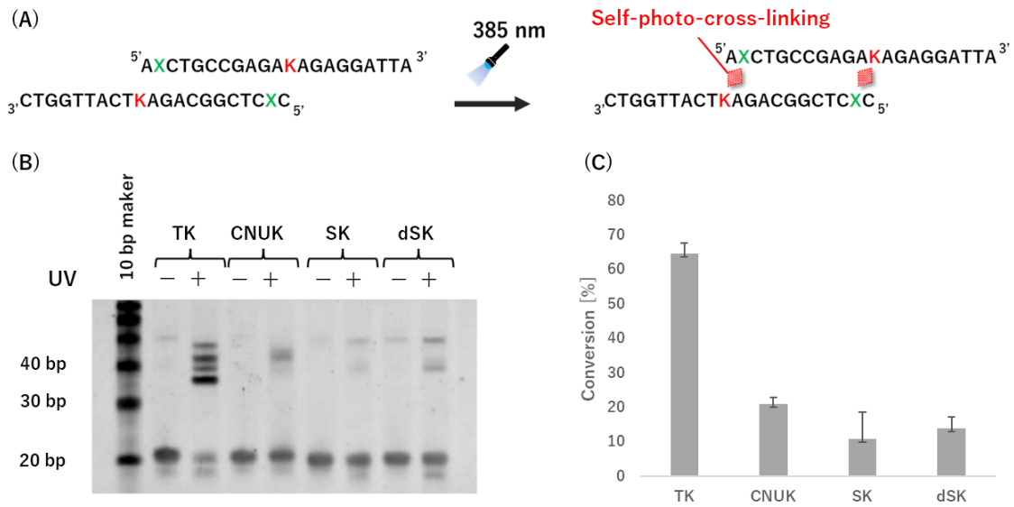
Figure 3.4. (A) Self-photo-cross-link inhibition scheme between antigen. (B) Denaturing PAGE analysis of self-photo-cross-linking. The antigen probe 5 \mu M in 50 mM Tris-HCl (pH 7.5) was incubated at 37 ^{\circ} C, 1 h, and 385 nm photoirradiation was performed at 37 ^{\circ} C for 15 min. (C) SYBR Gold images were obtained by LAS-3000 and band intensity was determined by ImageJ software. Self-photo-cross-linked efficiency was calculated by the average ratio of shifted band.
