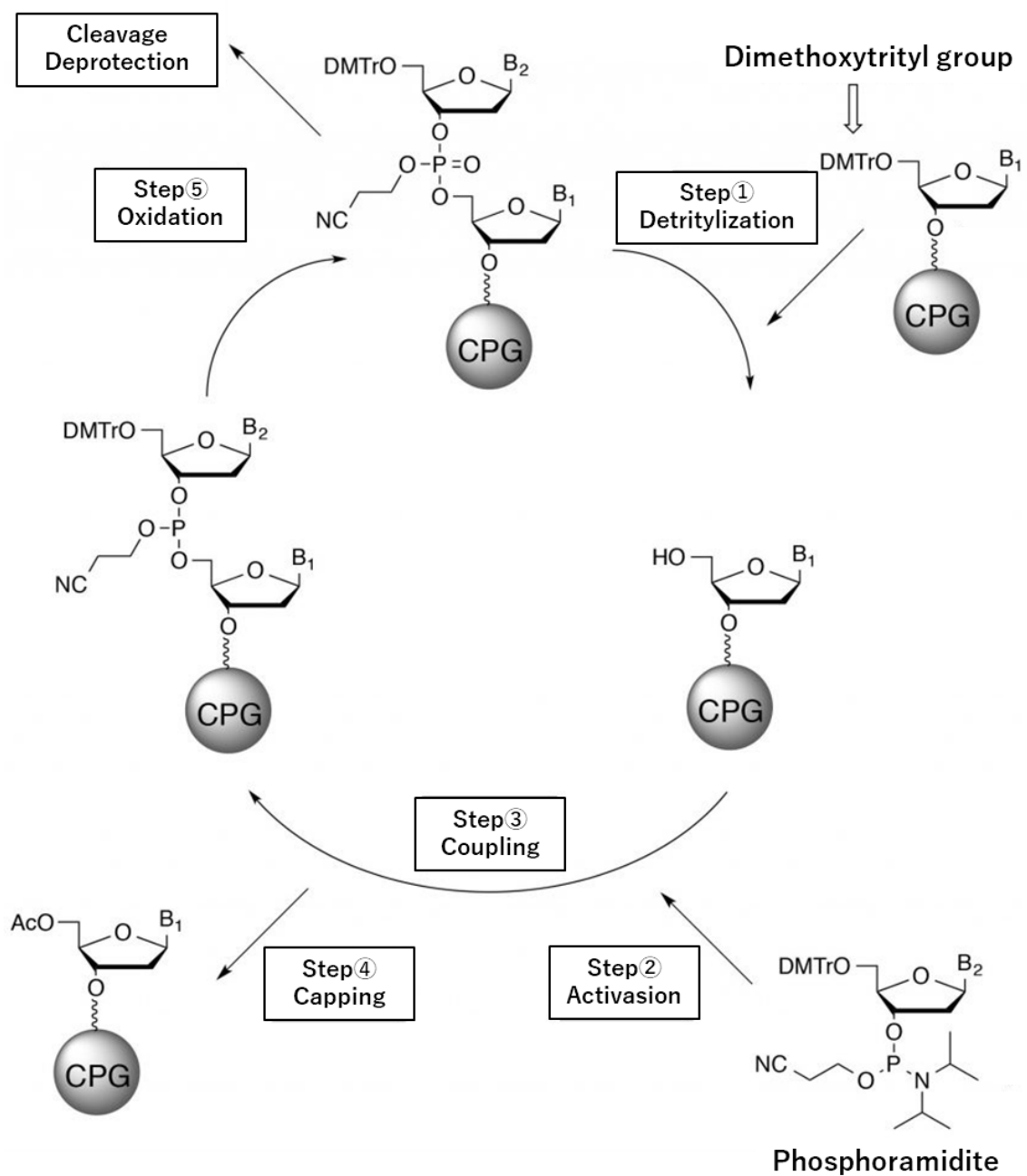
Figure 1.9. Phosphoramidite method
