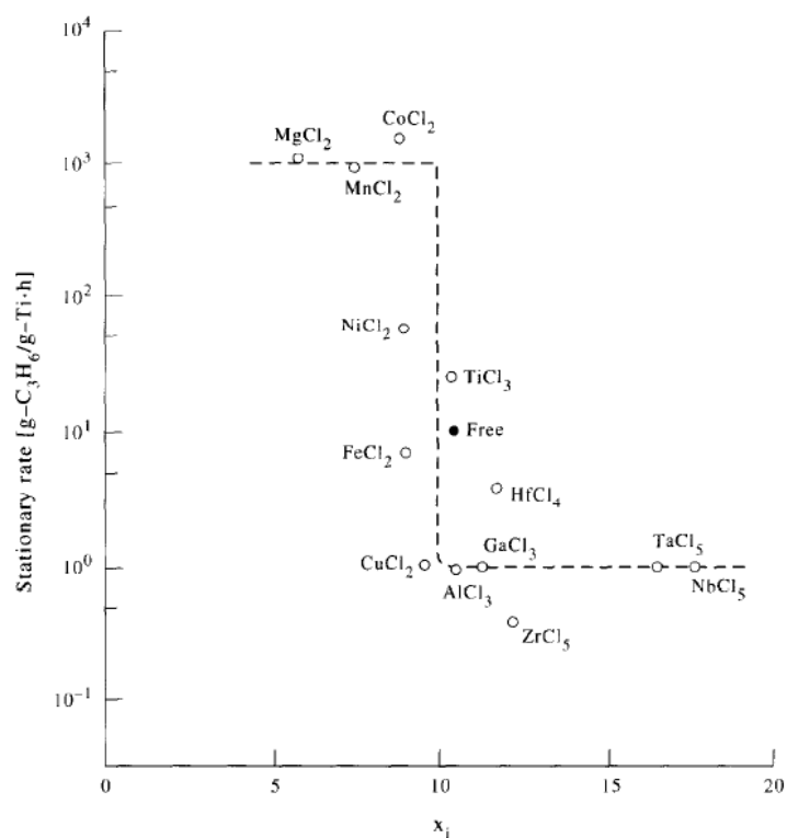
Figure 1.2. Electroactivity and steady state activity of metal ions.
