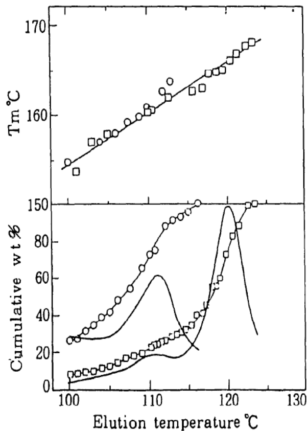
Figure 1.4. Cumulative and differential elution curves and melting point of the eluted polymer. (○) MgCl 2 -supported Ti-AlEt 3 system, (□) MgCl 2 -supported Ti-AlEt 3 - p -toluic acid methyl ester system
