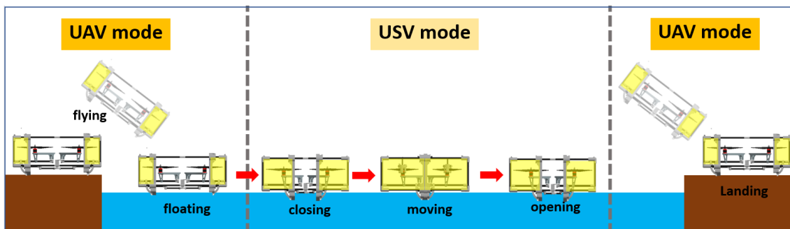
Fig. 1. An exemplary deployment scenario of a VTOL (vertical take-off and landing) UAV-USV hybrid vehicle outfitted with the transformable housing: flying offshore in UAV mode, navigating on the water surface in USV mode, and returning onshore in UAV mode.
