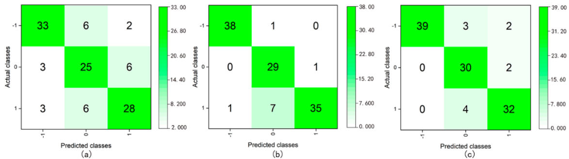
Figure 4.12 Confusion matrices of the ternary class classification using DT C5.0 (boosting) (a), RF (bagging) (b), and ANN (boosting) (c).
