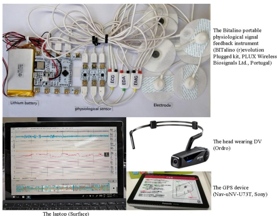
Figure 3.4 Data collection device: a Bitalino portable physiological signal feedback instrument (BITalino (r)evolution Plugged kit, PLUX Wireless Biosignals Ltd., Portugal), a head-wearing DV(Ordoro), a GPS device (Nav-uNV-U73T, Sony), and a laptop (Surface).
