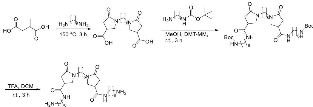
Scheme 4-1 Synthesis of bio-based bis-pyrrolidone diamines from itaconic acid.
