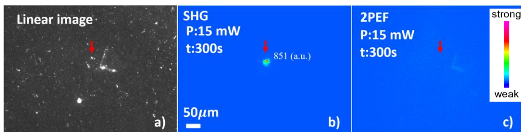
Figure 51. Linear, SHG, and 2PEF images of the original 0.5 wt% sacran solutions (13 spots)
