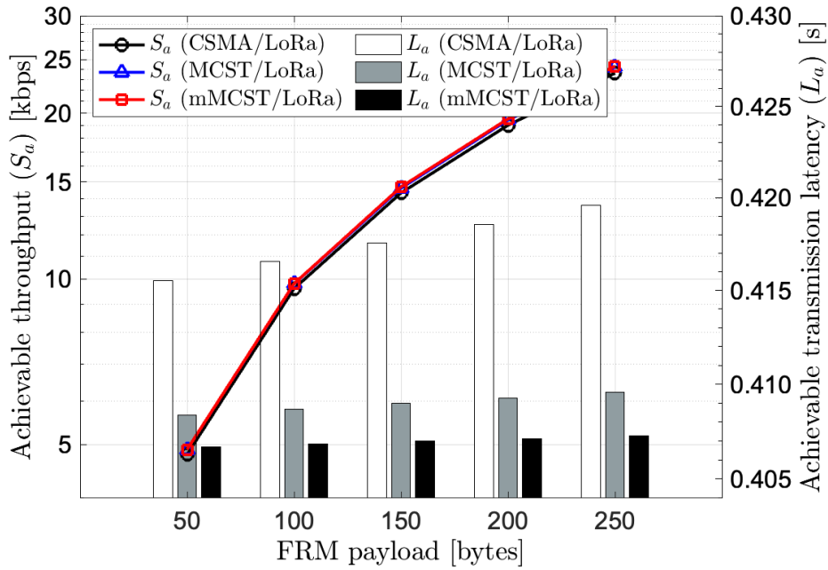
Figure 3.25: Performance comparison in average achievable throughput and latency for 30-node random network
