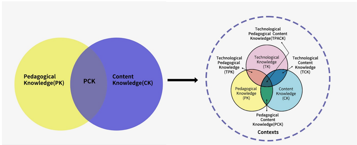
Figure 2 PCK model
