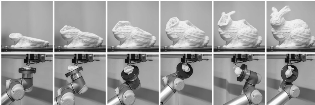
Fig. 4.3 Support-Free Volume Printing by Multi-Axis Motion [103]
