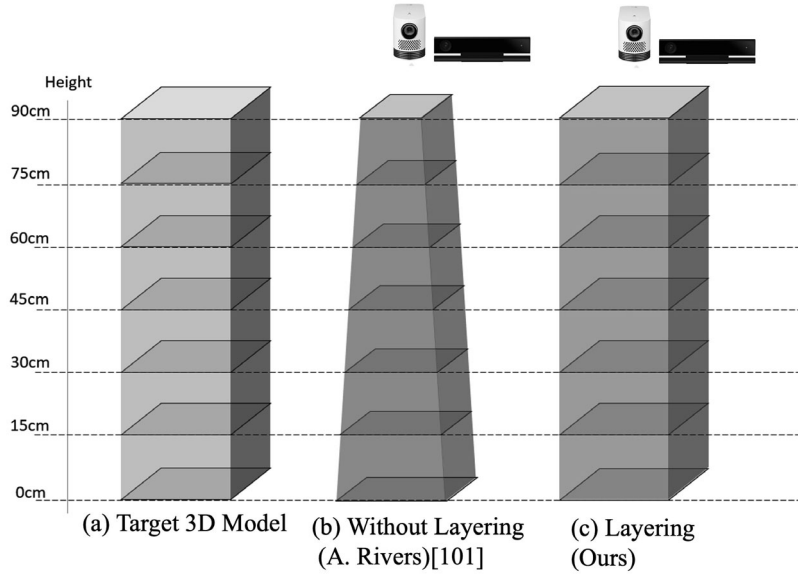
Fig. 4.10 The comparison of target 3D model. The model on the left shows a 50cm square target 3D model (a), and the shapes in the center and on the right represent the projected shapes of a target 3D model using existing methods and the proposed method. When projecting a target model using existing methods, the projected model becomes smaller as the height of the model increases (b). With our method, the size of the projected target model remains constant (c).
