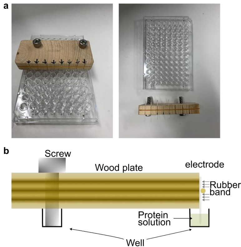
Fig. 5. Fixation method for safe oversight of the electrode tip. Electrodes are grabbed with tweezers and secured through rubber bands. Multiple electrodes can be attached at the same time. (a) A wood plate with electrodes fixed with rubber bands and a 96 well plate. By placing two screws in each well and fixing them in place, the entire wood plate is stuck and can be stored for a long time without the tip of the electrode touching the walls or bottom of the well. In use (left) and disassembled (right). (b) Well and wooden board in use (Side view). Electrodes are always pressed by the rubber band.
