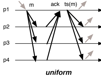
図 5.5: Destinations Agreement
