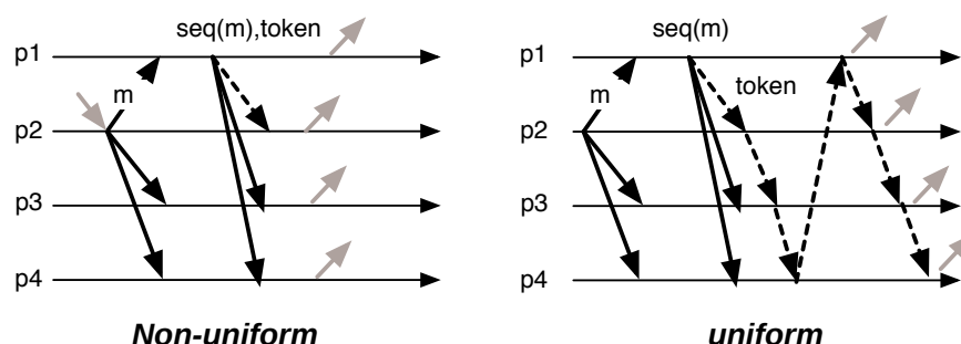
図 5.2: Moving Sequenser
