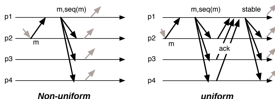
図 5.1: Fixed Sequencer
