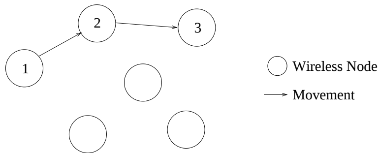
図 4.12: Random Waypoint
