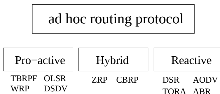
図 2.3: routing protocol
