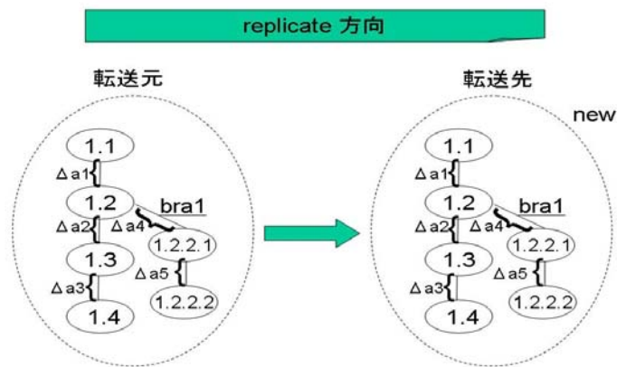
図 3.21: replicate
