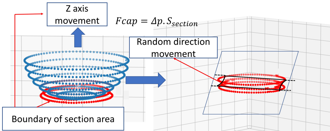
FIGURE 27: Tangential capillary force estimation following the wetted liquid and movement direction, where S_{section} is the projected area of the wetting liquid on a plane perpendicular to the direction of motion.
