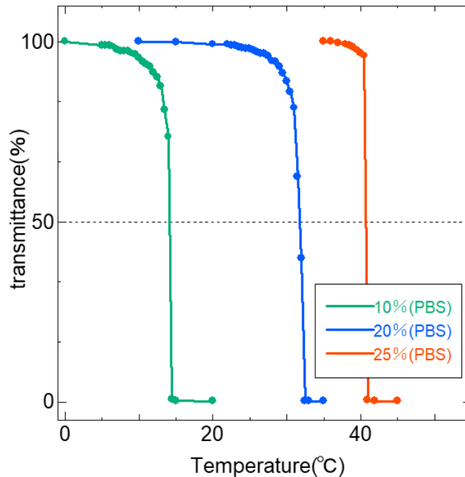
Figure 21 Changes in transmittance intensity across different temperature ranges (UV-vis, \lambda=550 nm; 50% transmittance indicates phase separation temperature) The phase separation temperatures for PLL-PA(-SH) at various concentrations in PBS.
