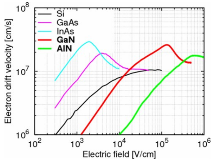
Figure 1.6: Relation between drift velocity and electric field obtained by Monte Carlo simulation [11].
