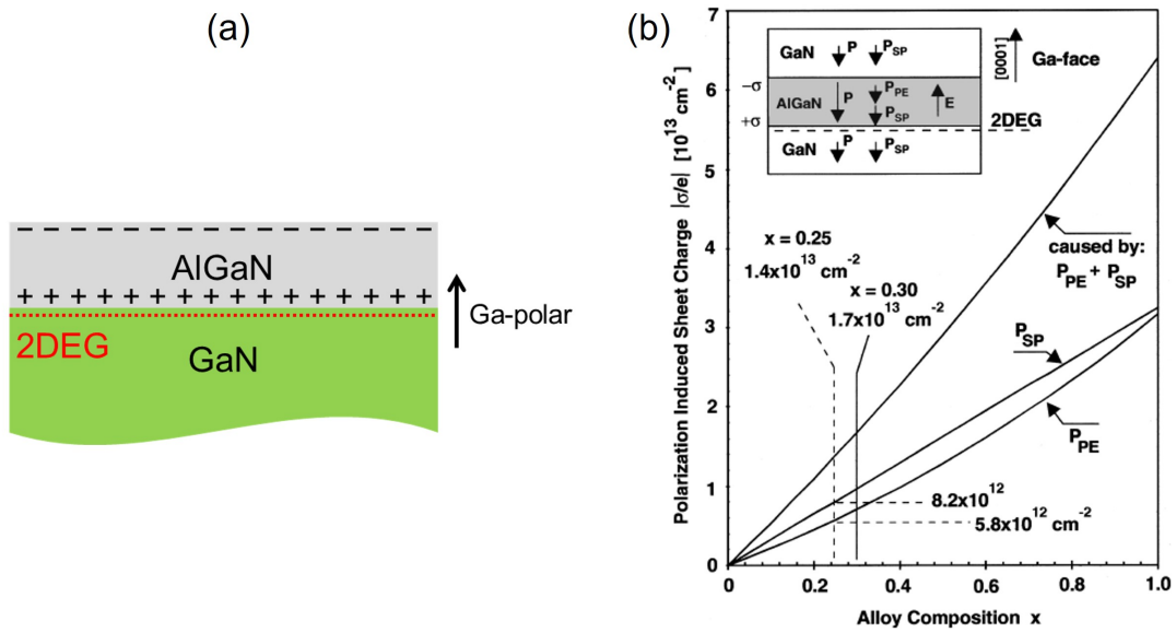
Figure 1.13: (a) The 2DEG at the AlGaN/GaN heterointerface. (b) Calculated sheet charge density caused by spontaneous and piezoelectric polarizations of a GaN-face GaN/AlGaN/GaN heterostructure [18].
