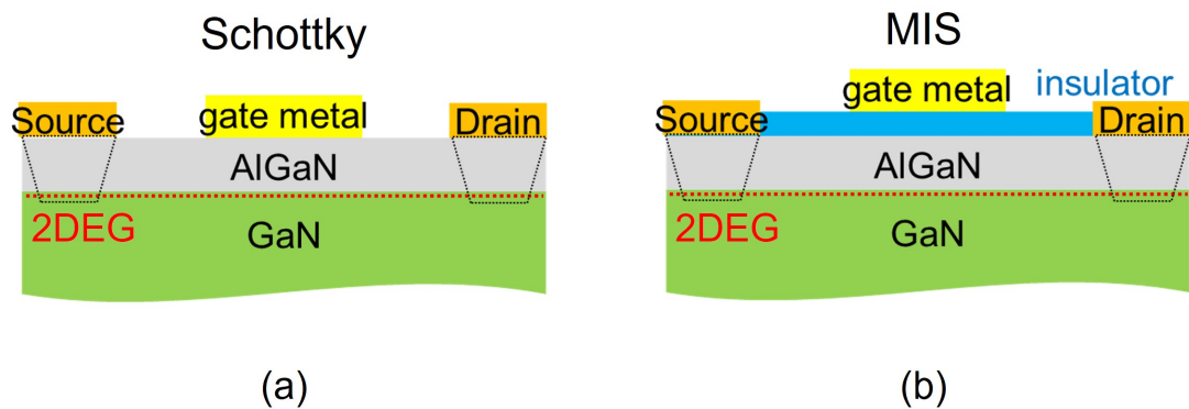
Figure 1.14: (a) A schematic cross section of AlGaN/GaN Schottky FETs. (b) A schematic cross section of AlGaN/GaN MIS FETs.
