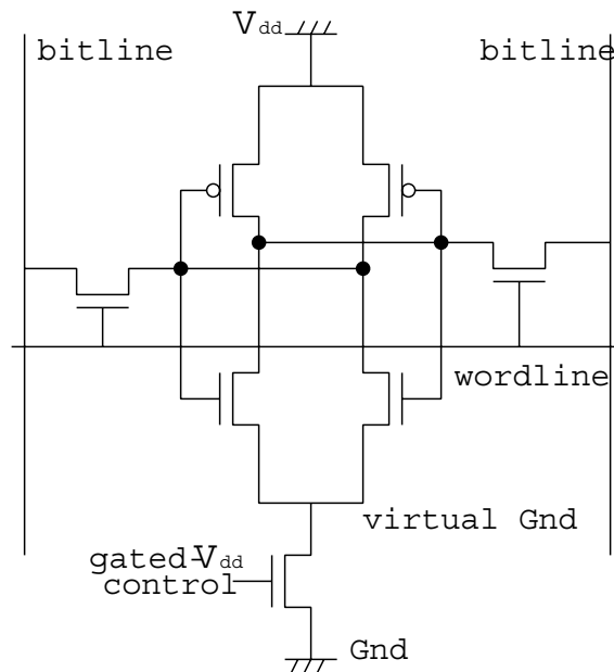
図 5.1: NMOS Gated-Vdd
