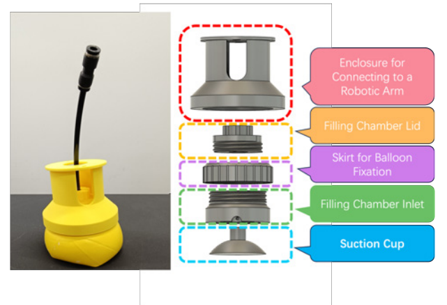
Fig. 2: Suction Cup Structure.
