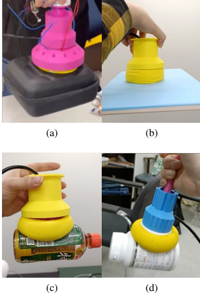
Fig. 3: Successful adhesion of the suction cup to different objects: (a) a box with engraved text, (b) a textured cutting board, (c) a bottle with an uneven surface, and (d) a relatively smooth paint bottle containing 1kg of coating material.
