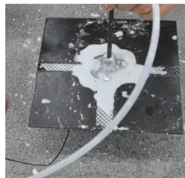
Fig. 1: The suction cup successfully adhered to the PLA board using a starch-water solution.
