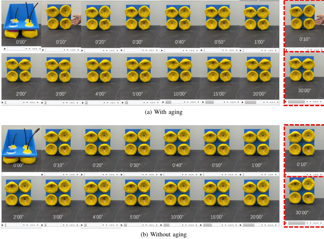
Fig. 8: The time-dependent deformation of the skirt under gravity.
